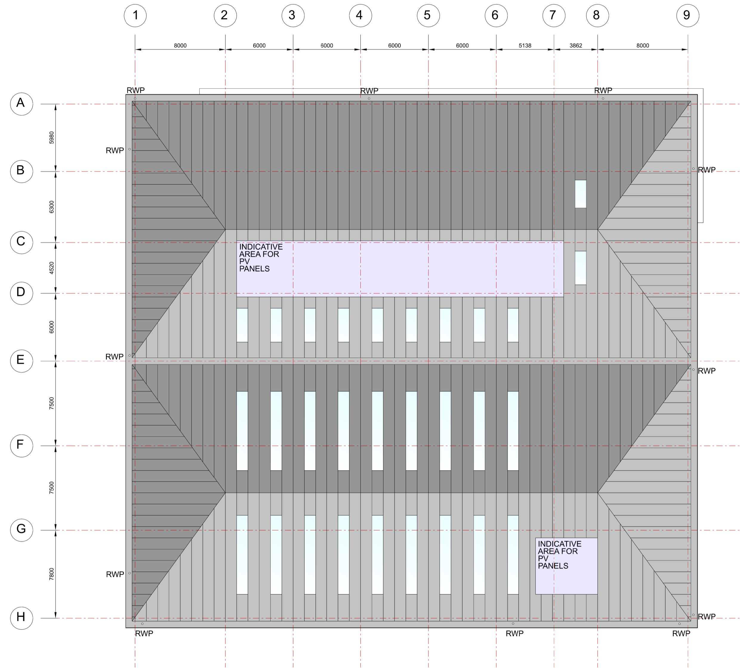
1 Unit 10 103 Roof Plan
