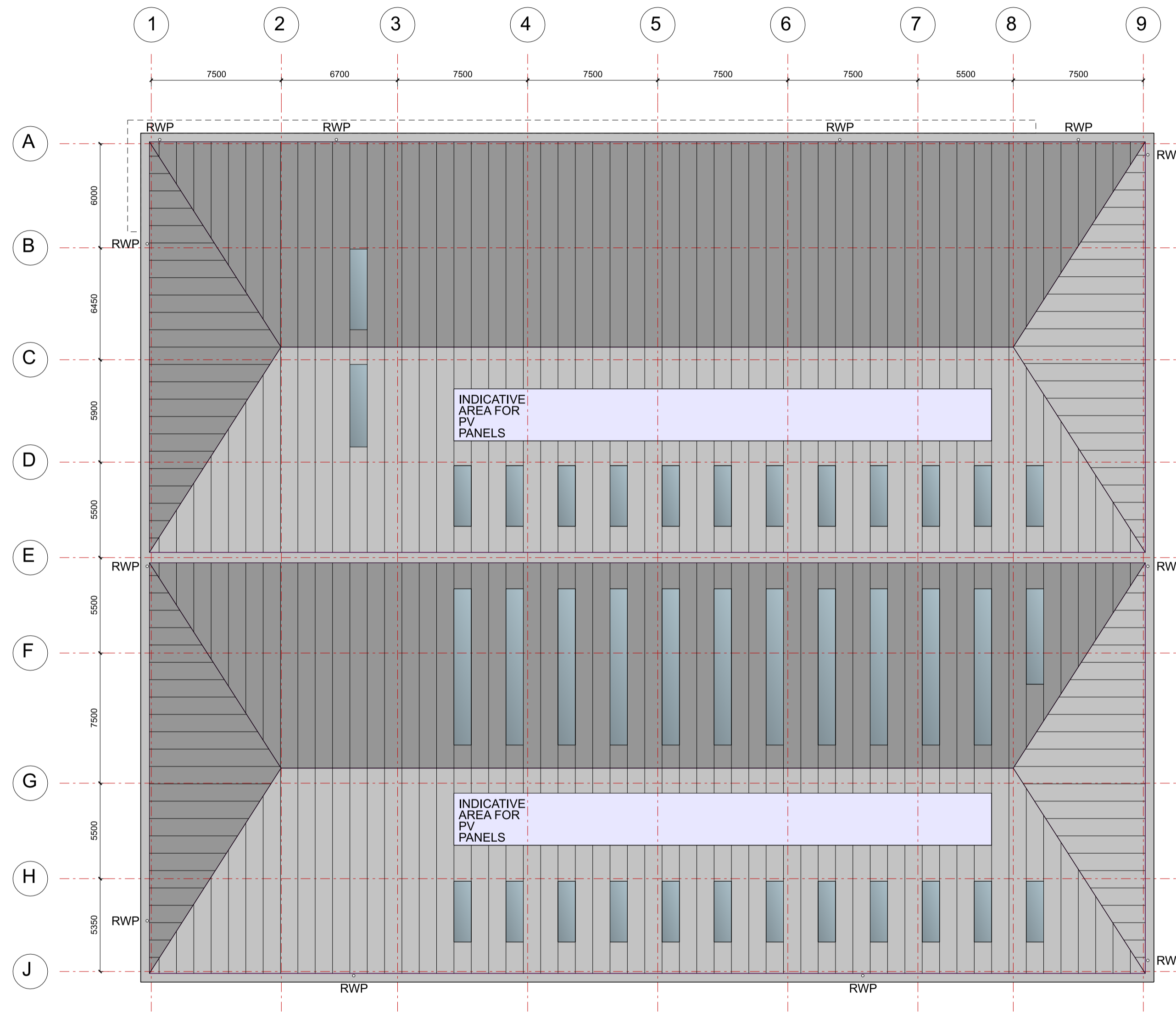
1 Unit 13 111 Roof Plan
