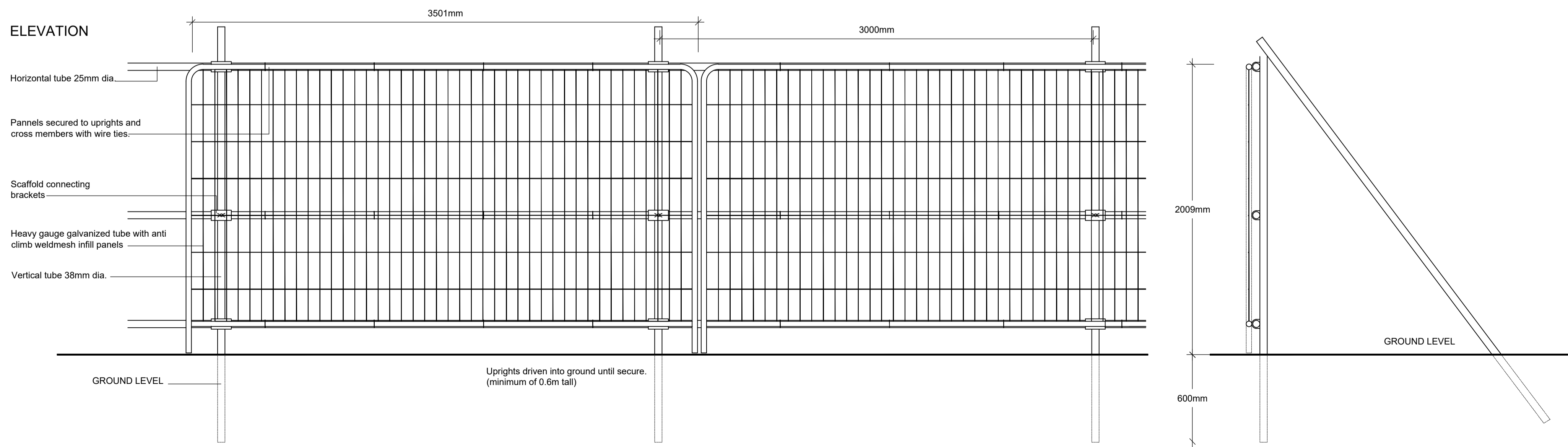
FIGURE 1) HERAS TYPE PANEL PROTECTIVE FENCING (ON STEEL SCAFFOLD FRAMEWORK) SCALE 1:20
