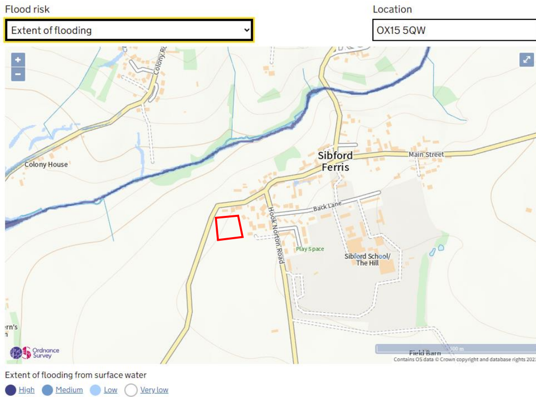
Figure 3: Surface Water Mapping
