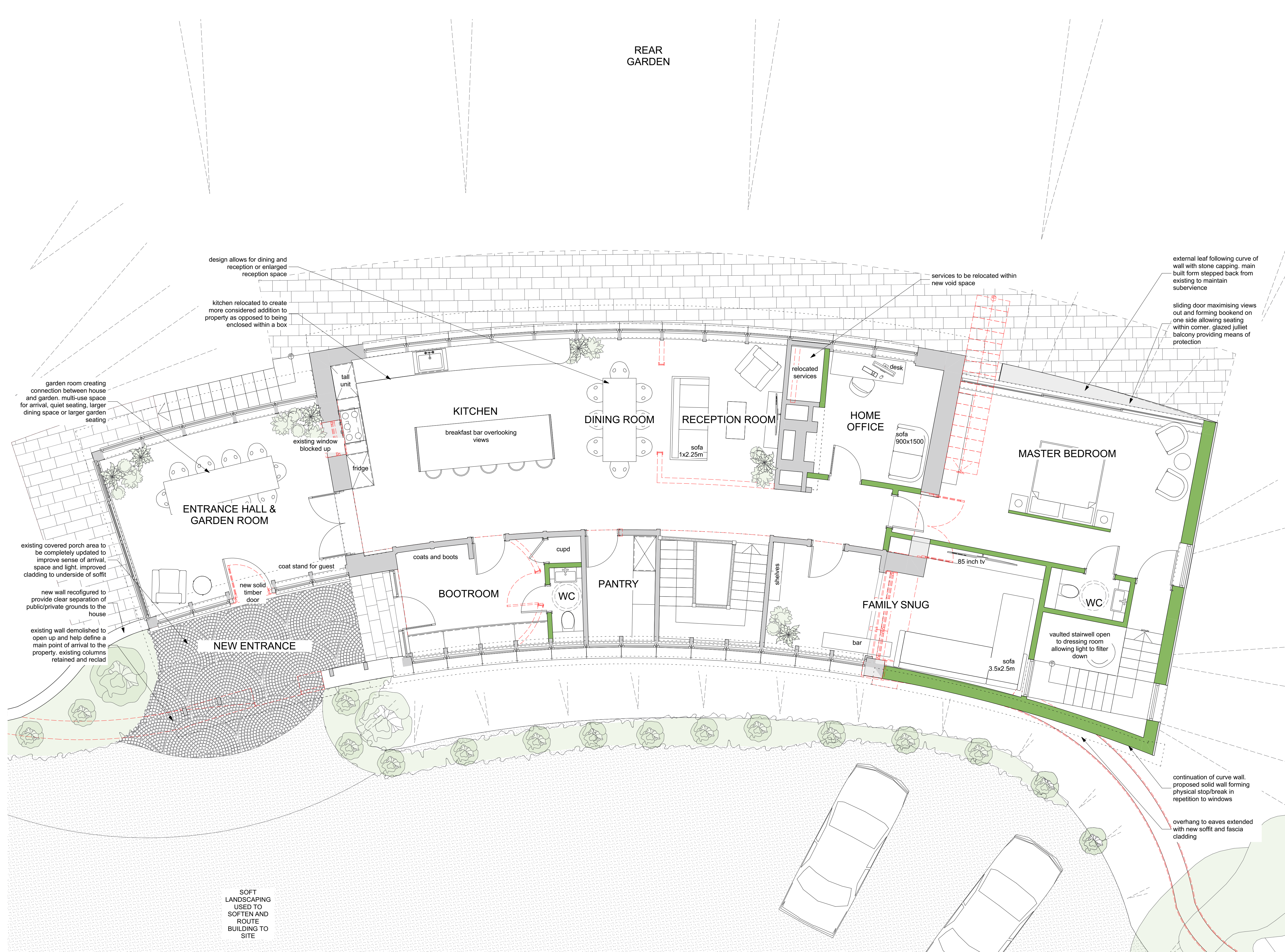
PROPOSED UPPER FLOOR PLAN
