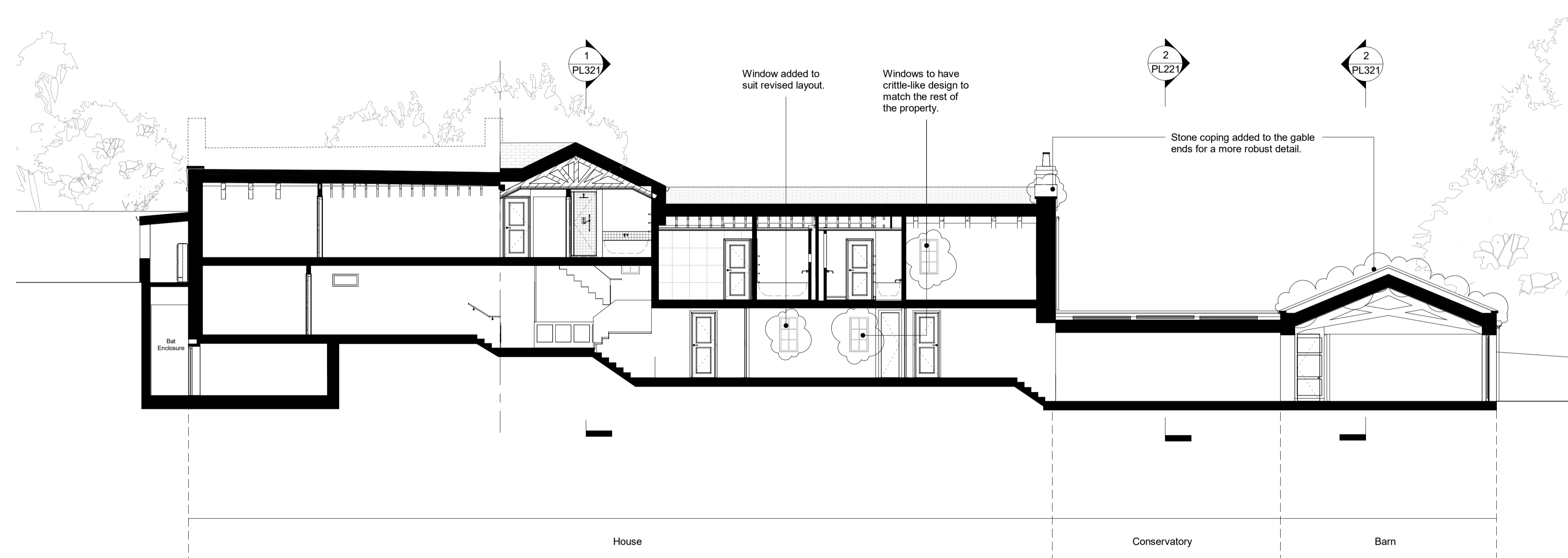
1 Proposed Section AA 1 : 100
