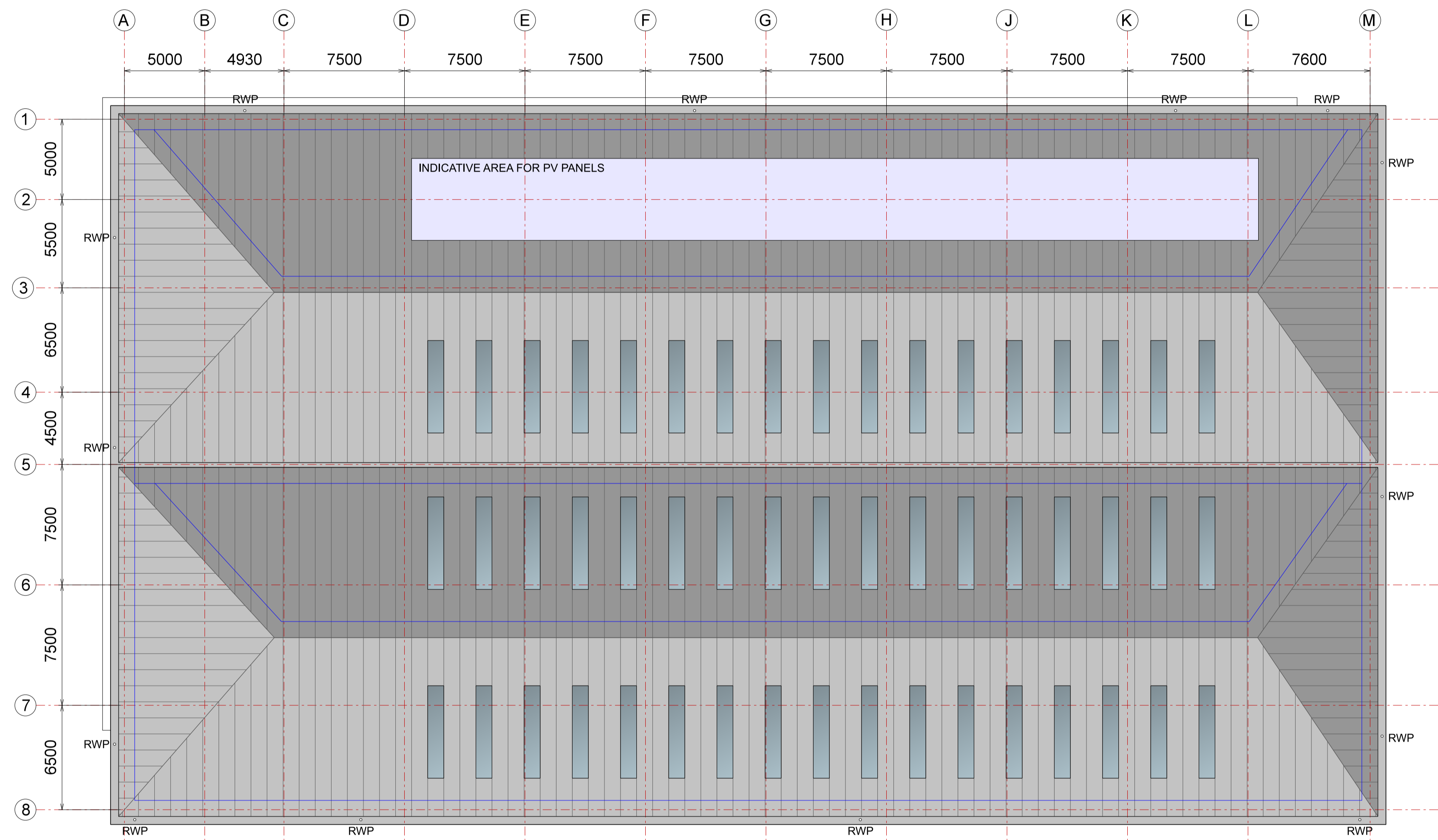
1 Unit 5b 007 Roof Plan
