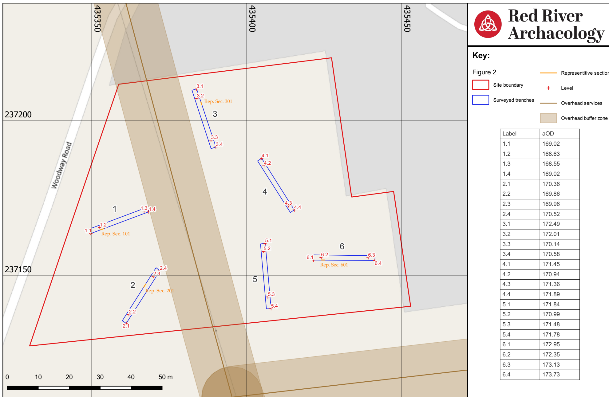
Figure 2 - Surveyed trenches showing levels data and representative section locations
