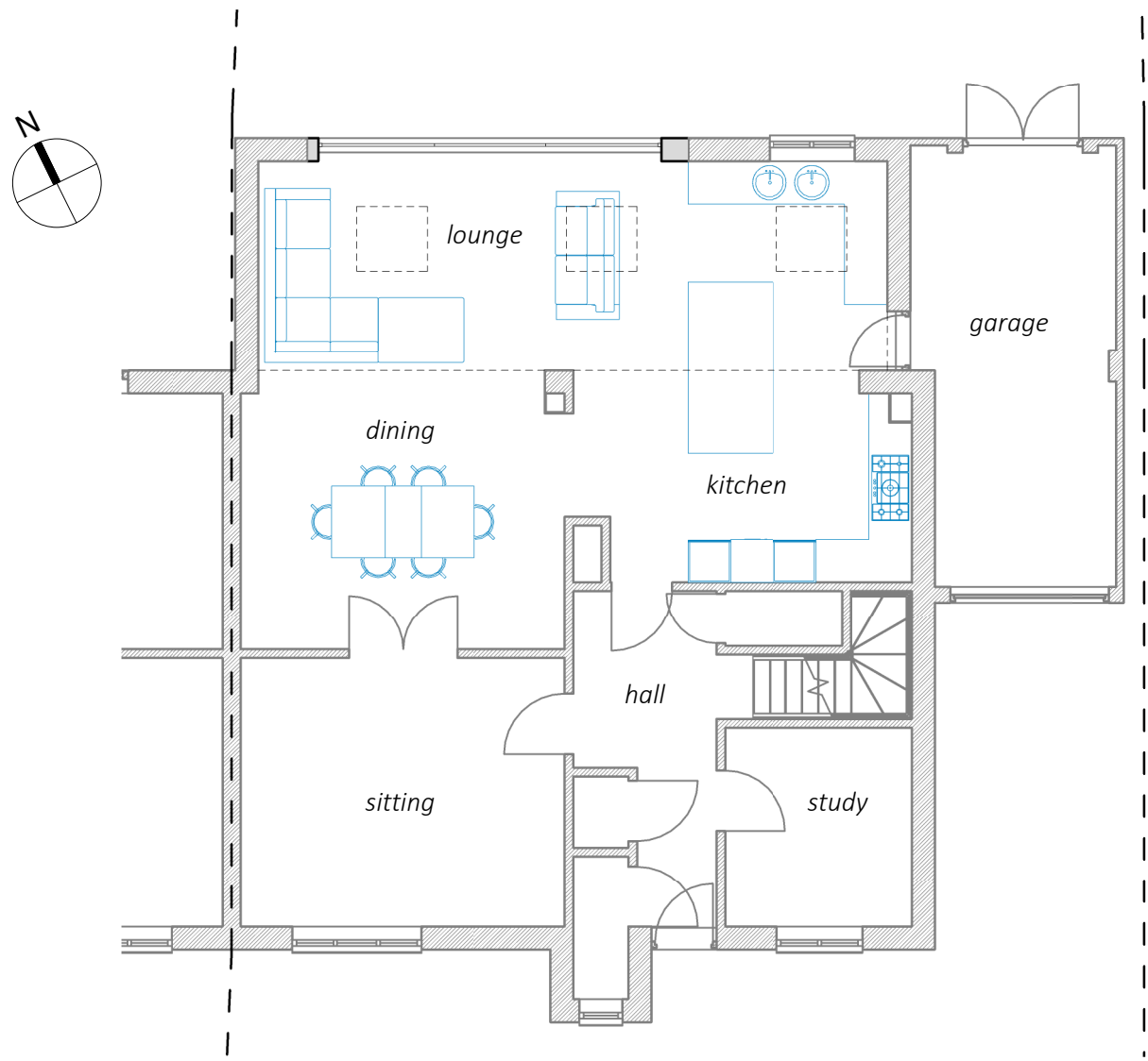
1 P3.2 Ground floor as proposed P05 1 : 100
