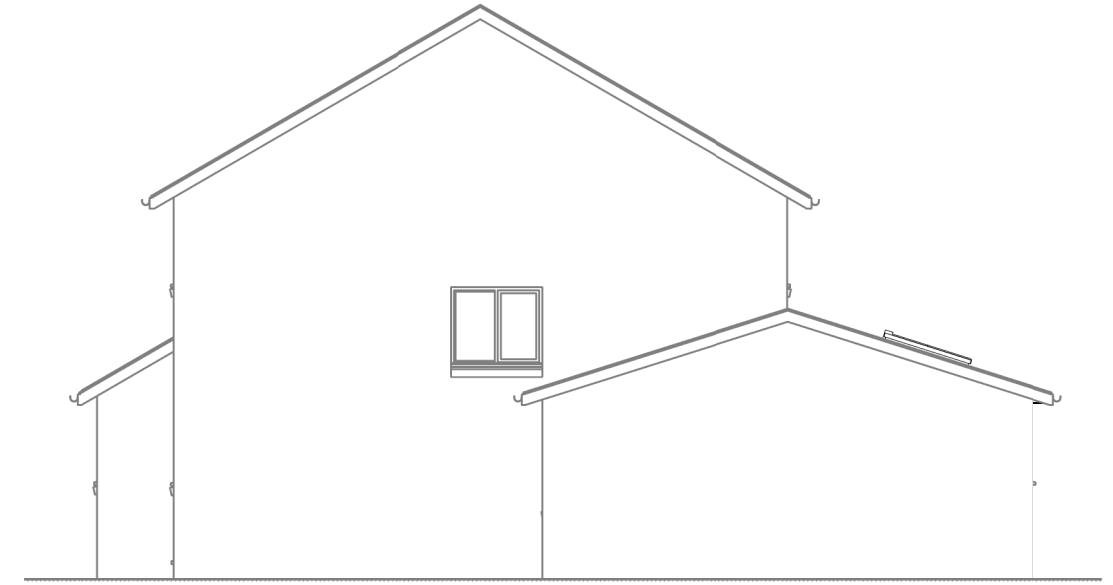
2 P06 ESE elevation - proposed 1 : 100
