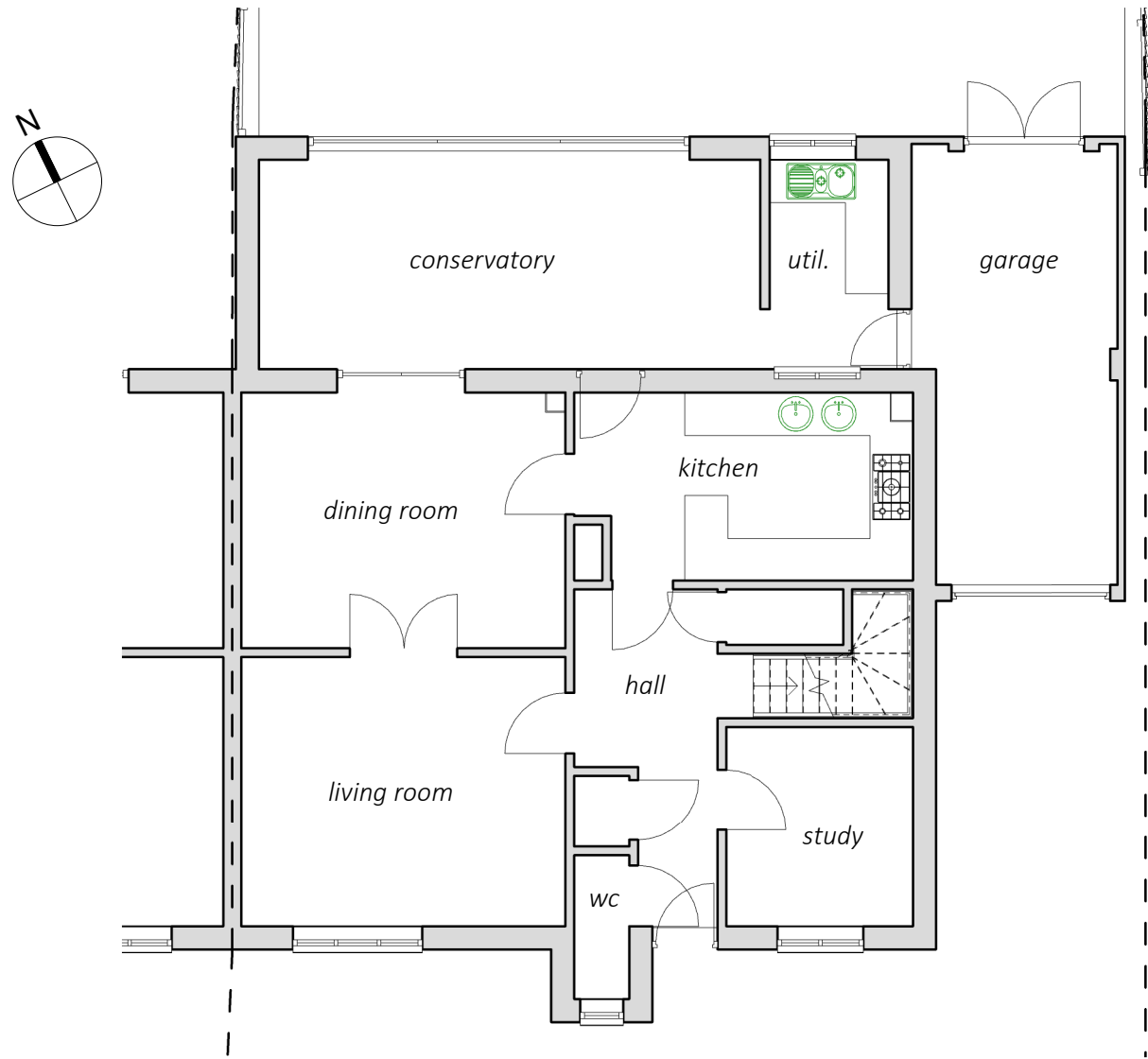
1 P02 P3.0 Ground floor as existing 1 : 100
