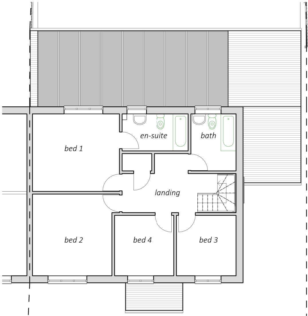
2 P02 P4.0 First Floor as existing 1 : 100
