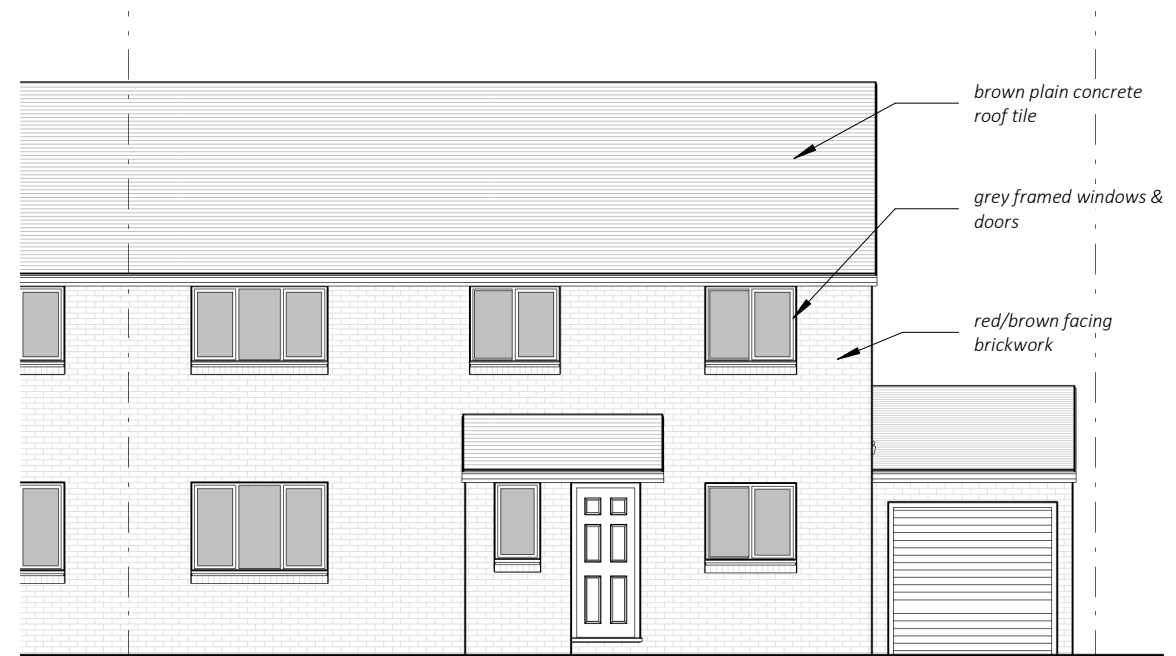
4 SSW elevation - existing P04 1 : 100
