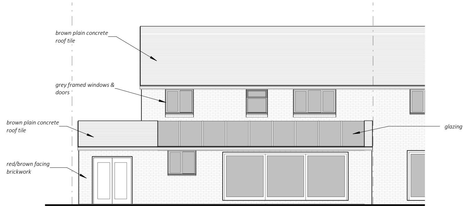
1 NNE elevation - existing P04 1 : 100
