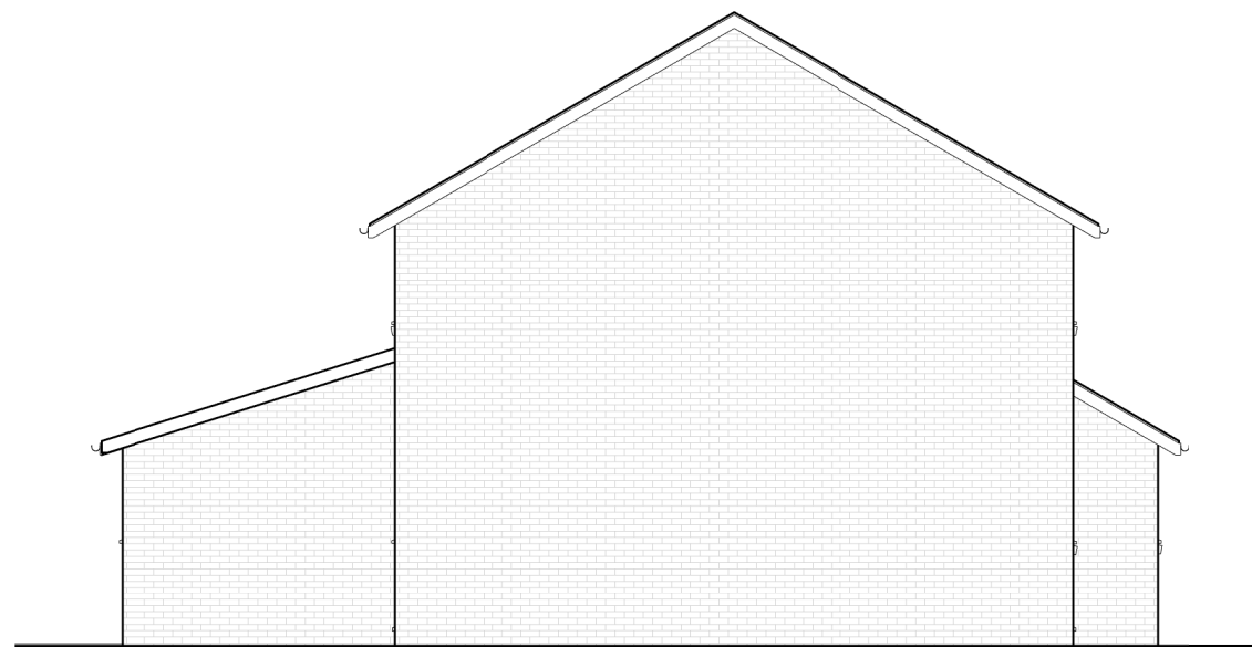
3 WNW elevation - existing P04 1 : 100
