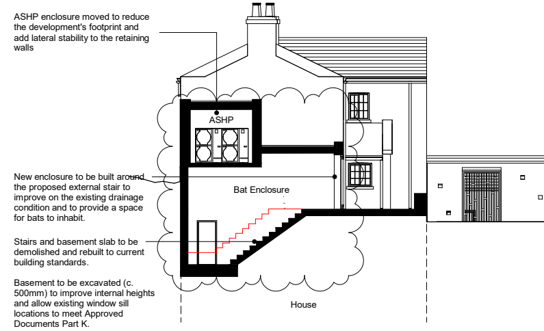
1 Proposed West Elevation 1 : 100
