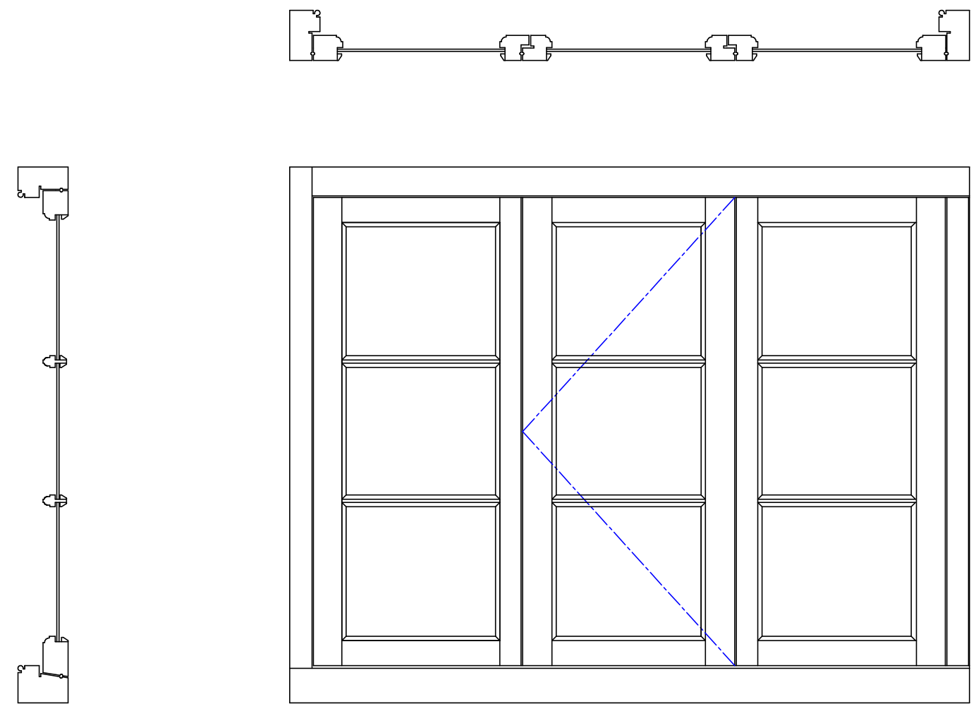
Kitchen Window Elevation & Section Through Scale 1:10 (@A2)
