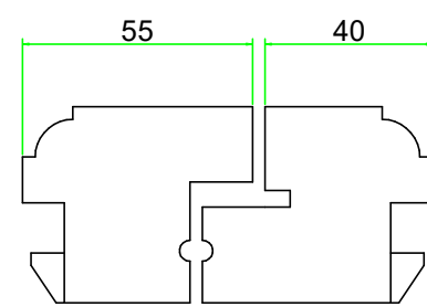
Casement Meeting Stile Section
