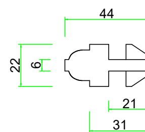
Glazing Bar Section
