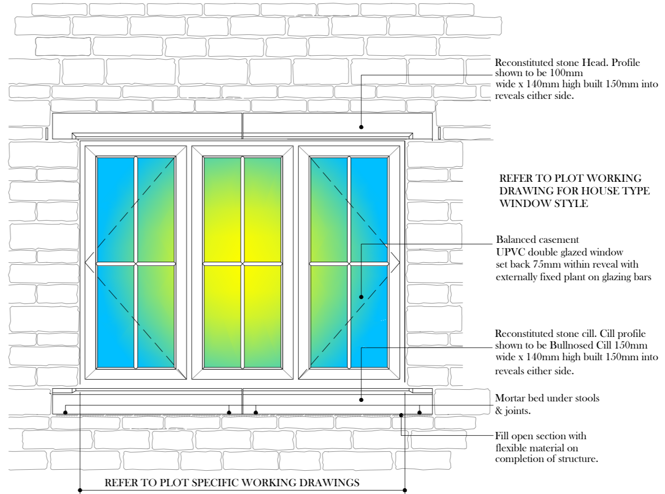
TYPICAL STONE ELEVATION WITH TWO PIECE STONE CILL AND LINTEL
