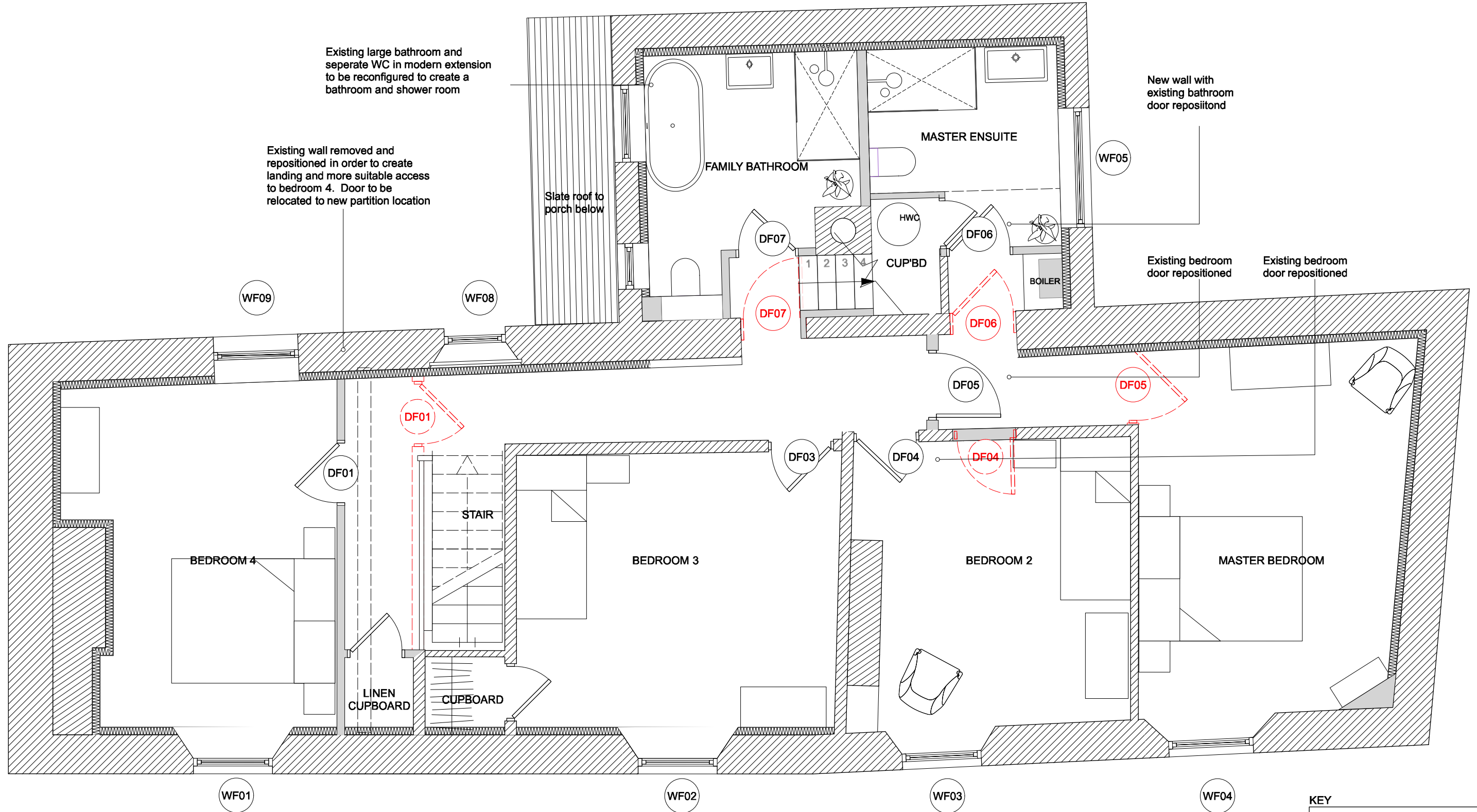
1 Proposed First Floor Plan Scale: 1:50
