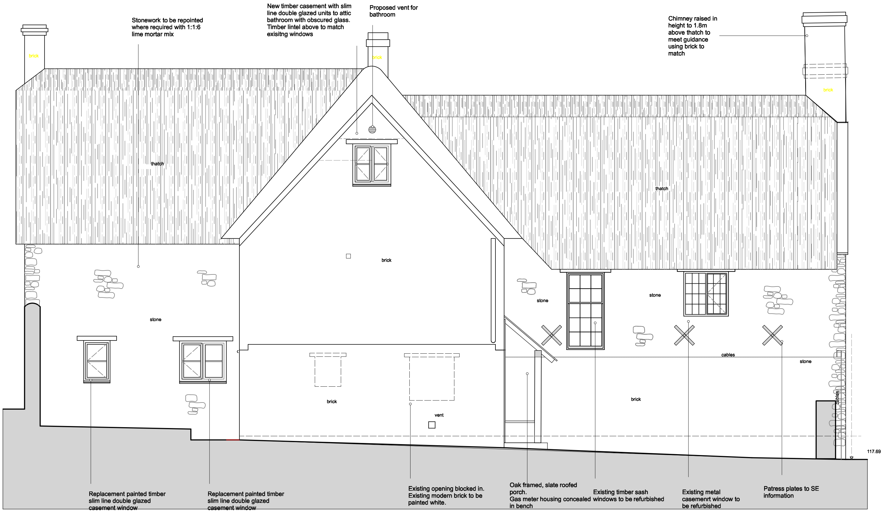
1 Proposed North Elevation Scale: 1:50
