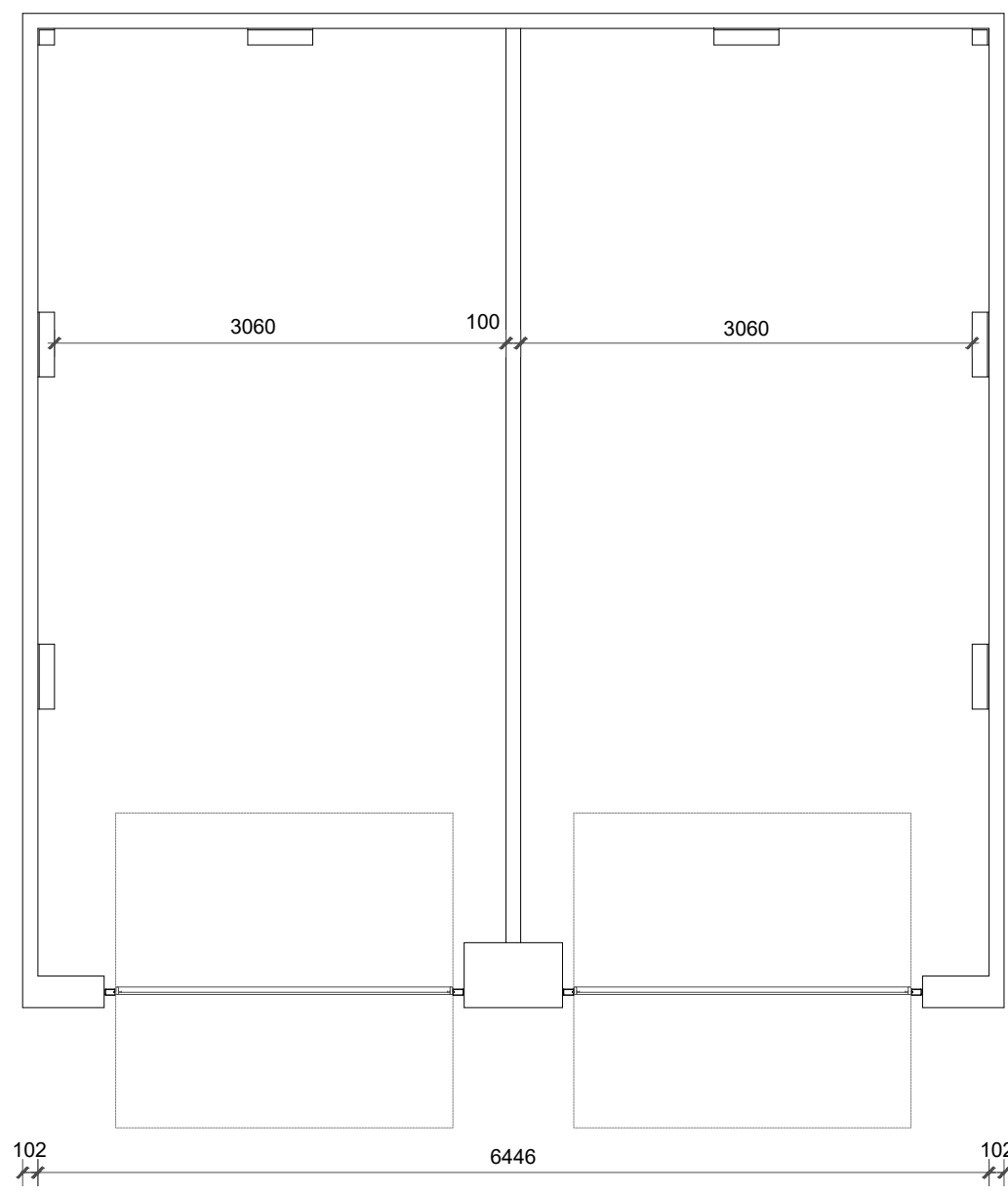
FLOOR PLAN
