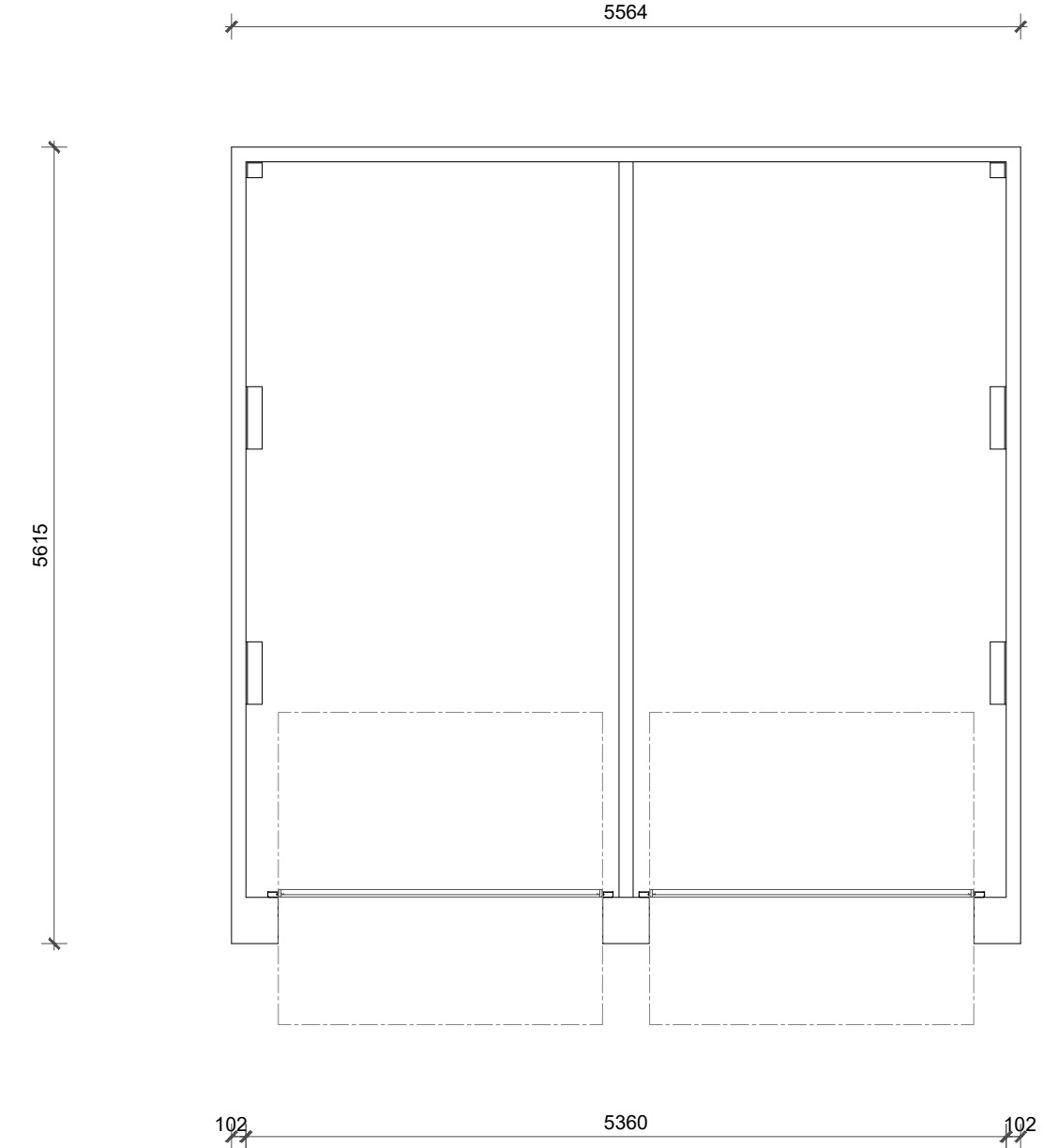
FLOOR PLAN
