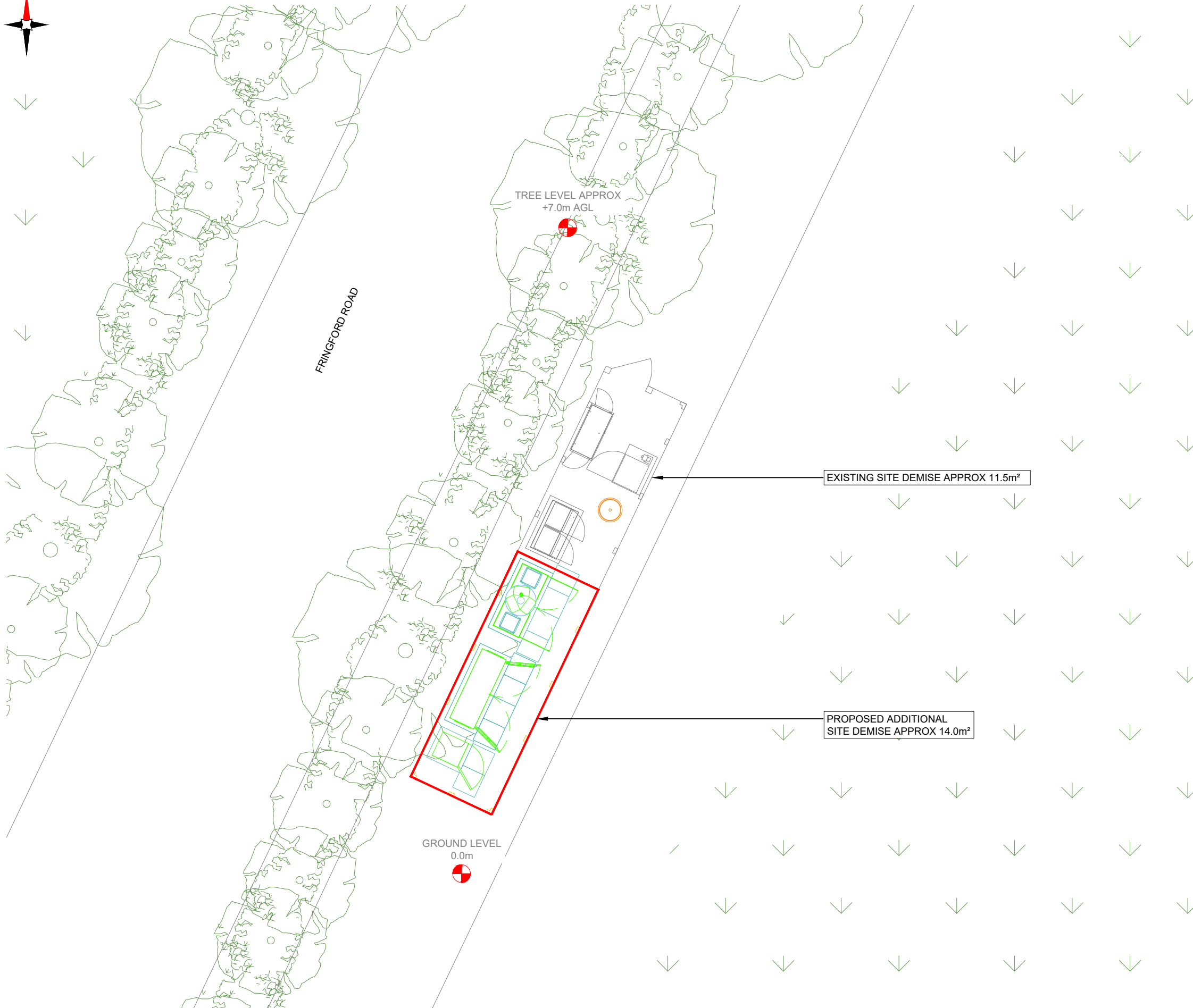
LEASE PLAN
