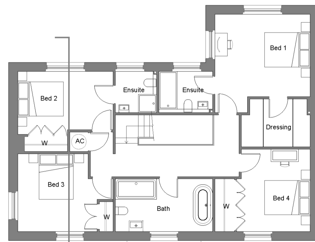
FIRST FLOOR PLAN 100sq.m.
