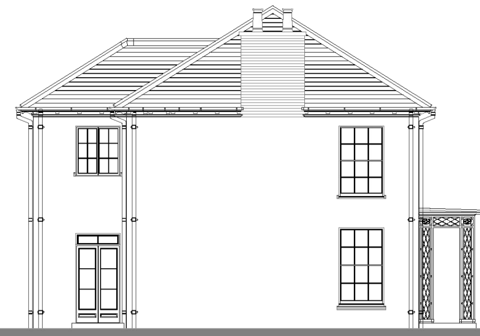
SIDE ELEVATION
