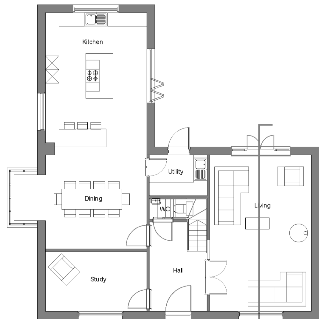
GROUND FLOOR PLAN 113sq.m.
