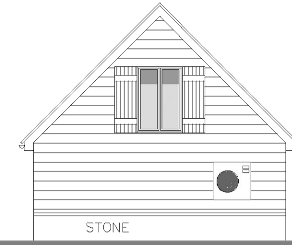
GARAGE ELEVATIONS
