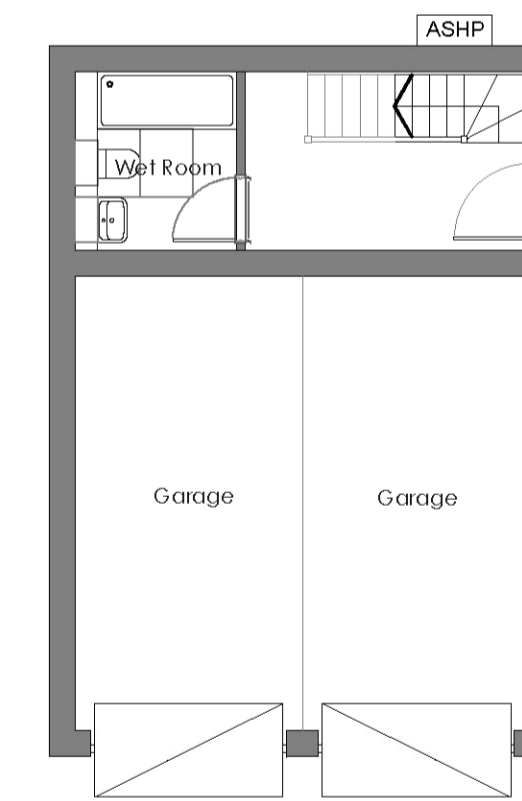
GARAGE PLANS
