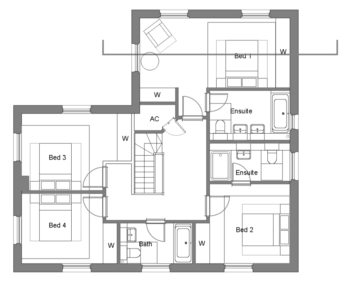
FIRST FLOOR PLAN 96.5sq.m.
