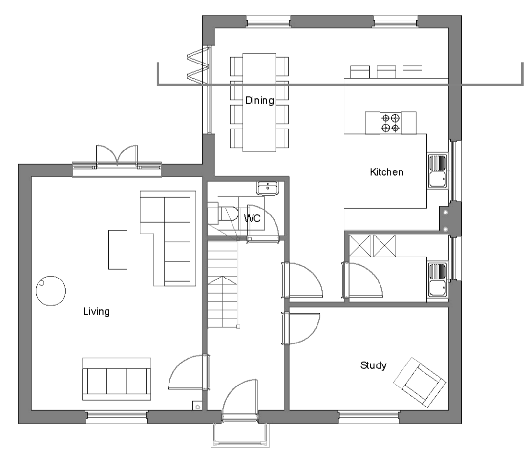
GROUND FLOOR PLAN 96.5sq.m.
