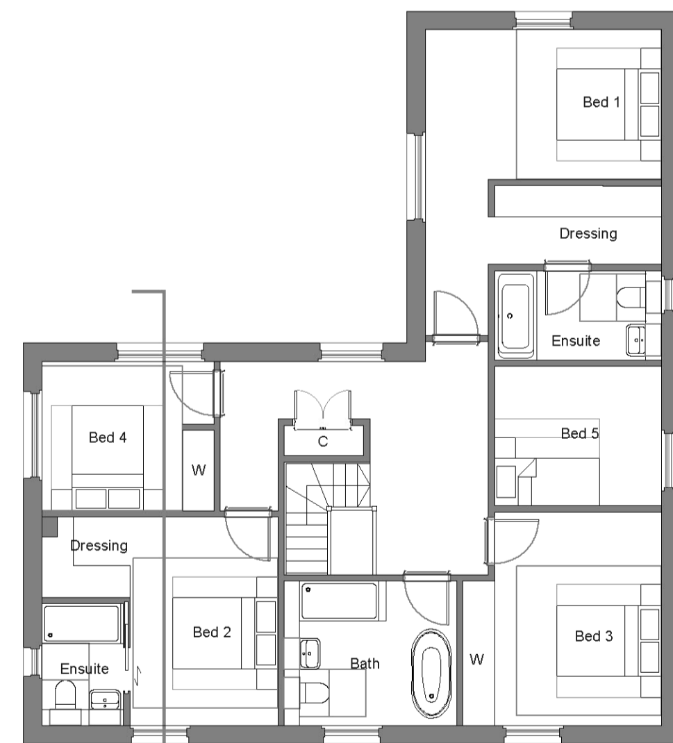
FIRST FLOOR PLAN 110sq.m.
