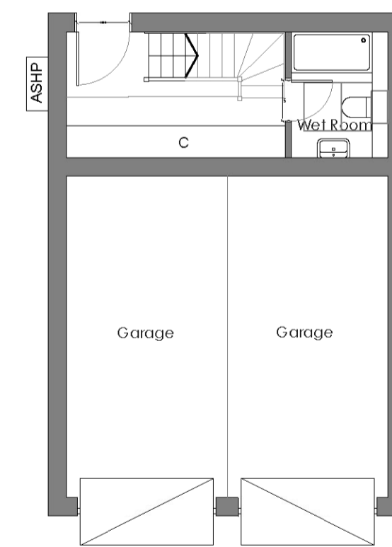
GARAGE PLANS
