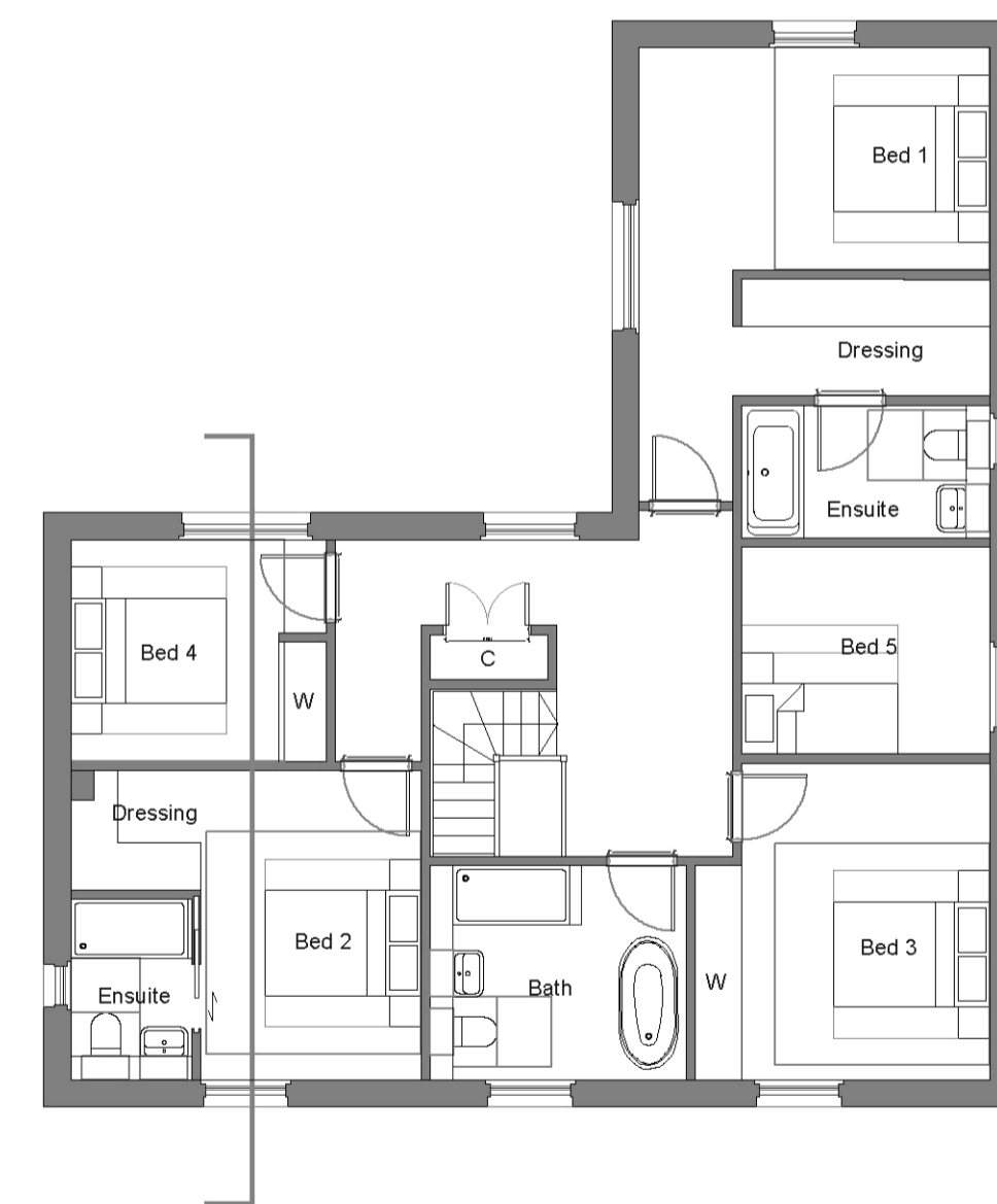
FIRST FLOOR PLAN 110sq.m.
