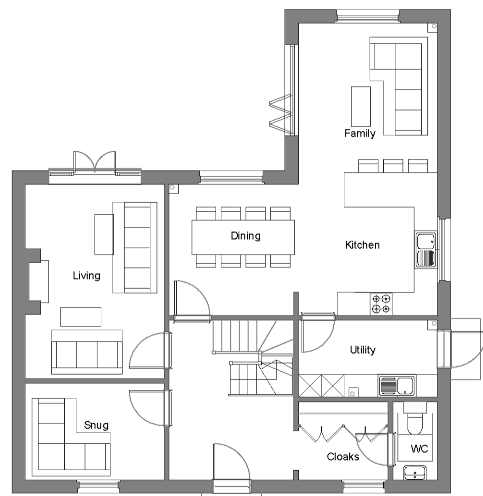
GROUND FLOOR PLAN 97.5sq.m.
