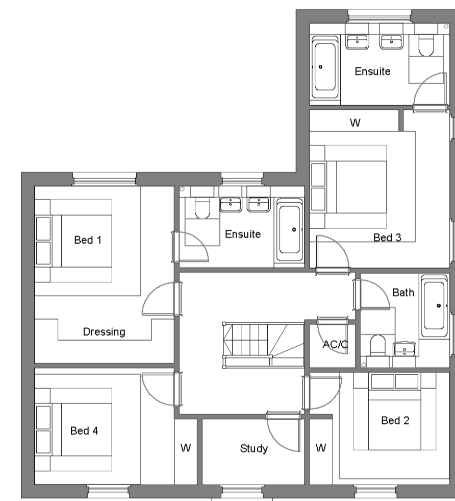
FIRST FLOOR PLAN 97.5sq.m.
