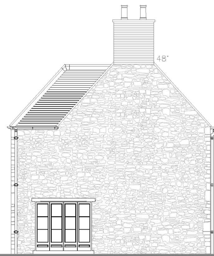
SIDE ELEVATION
