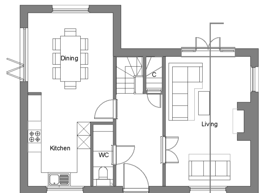
GROUND FLOOR PLAN 65.5sq.m.
