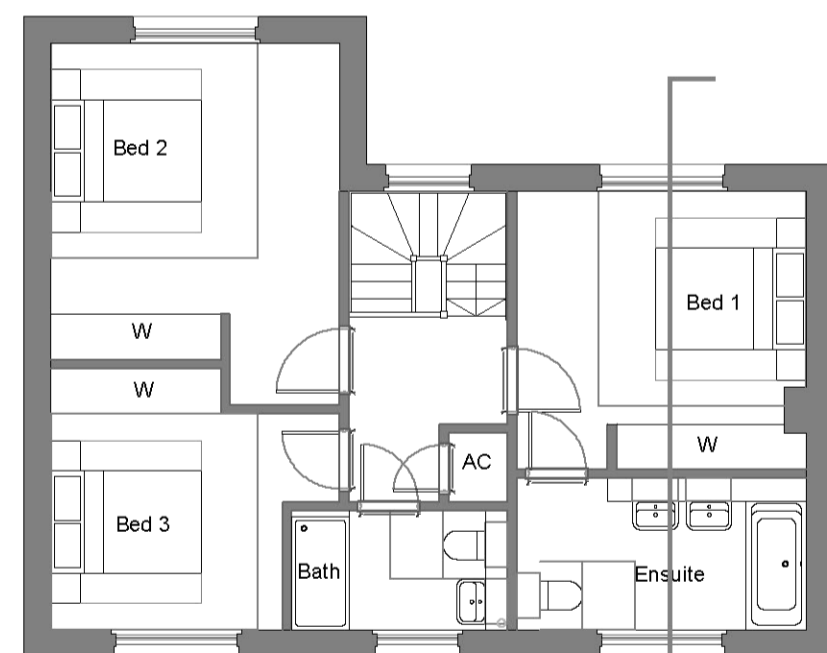
FIRST FLOOR PLAN 65.5sq.m.
