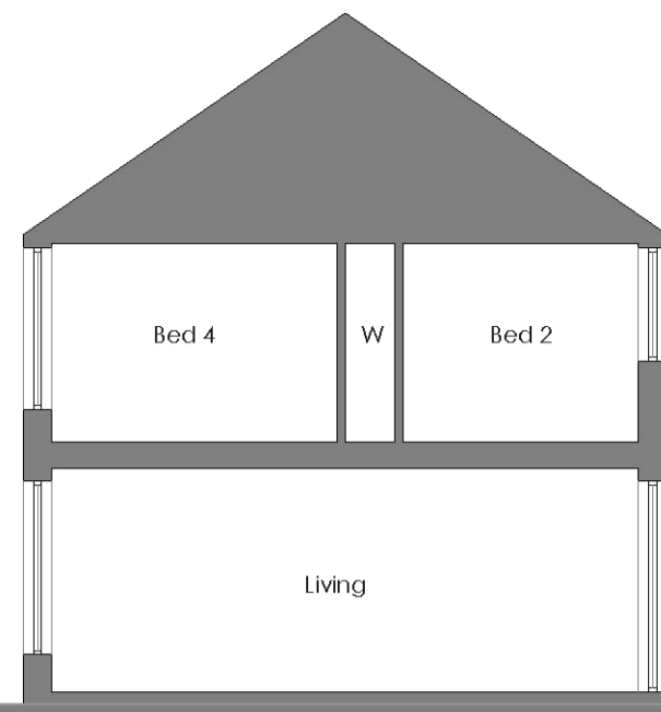
SECTION
