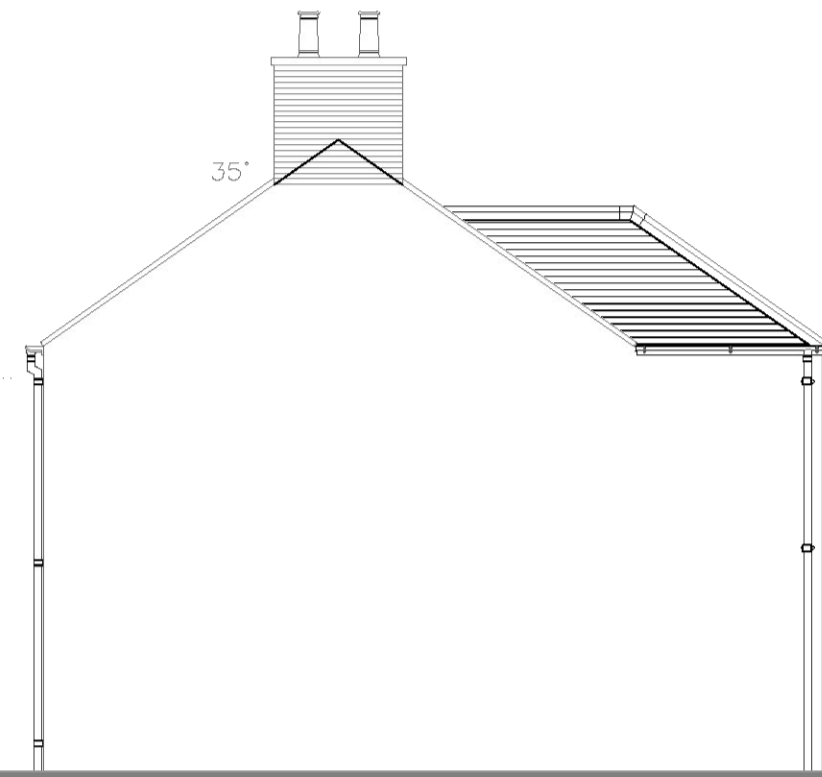
SIDE ELEVATION
