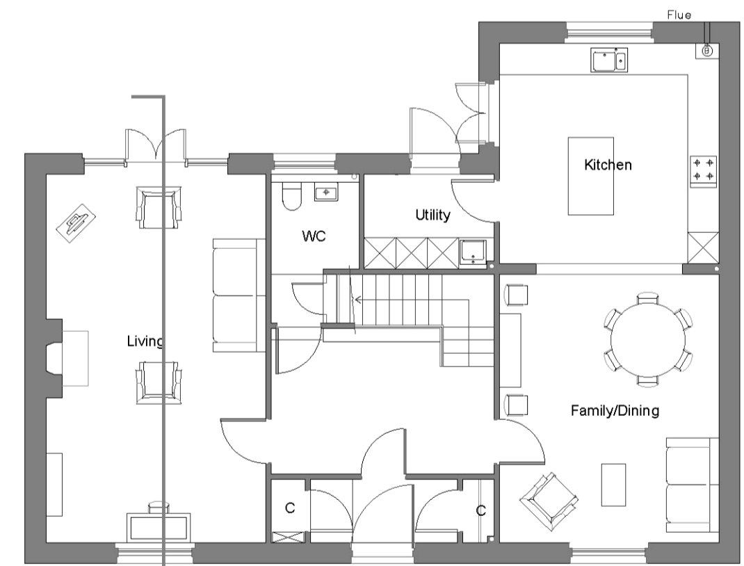
GROUND FLOOR PLAN 100sq.m.
