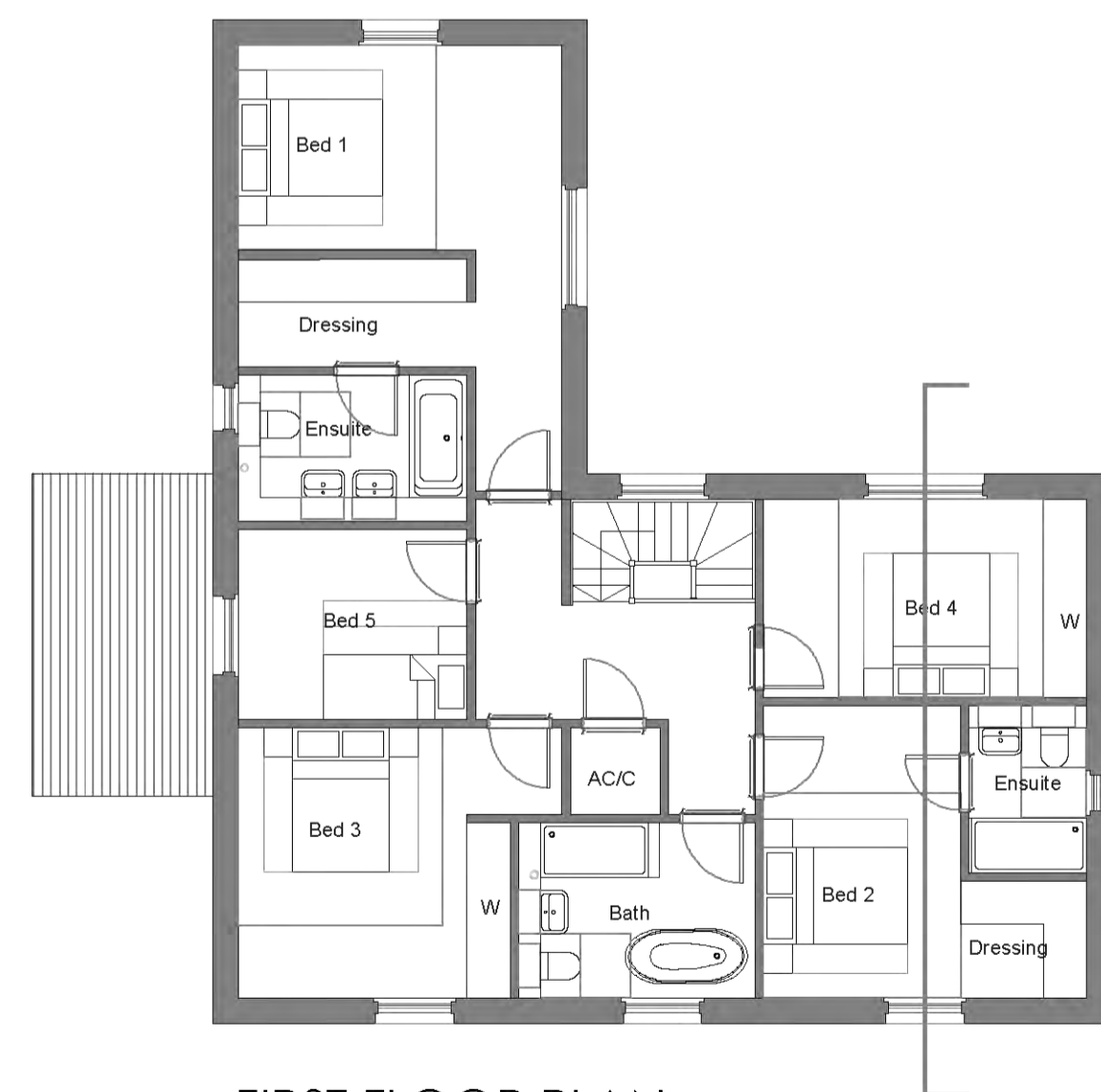
FIRST FLOOR PLAN 110sq.m.
