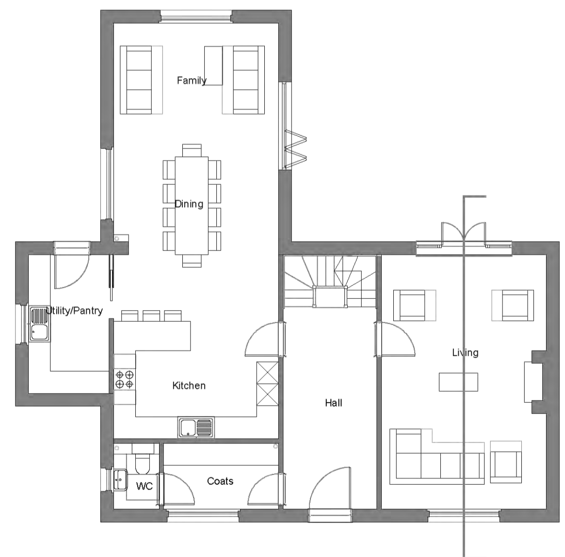
GROUND FLOOR PLAN 120sq.m.
