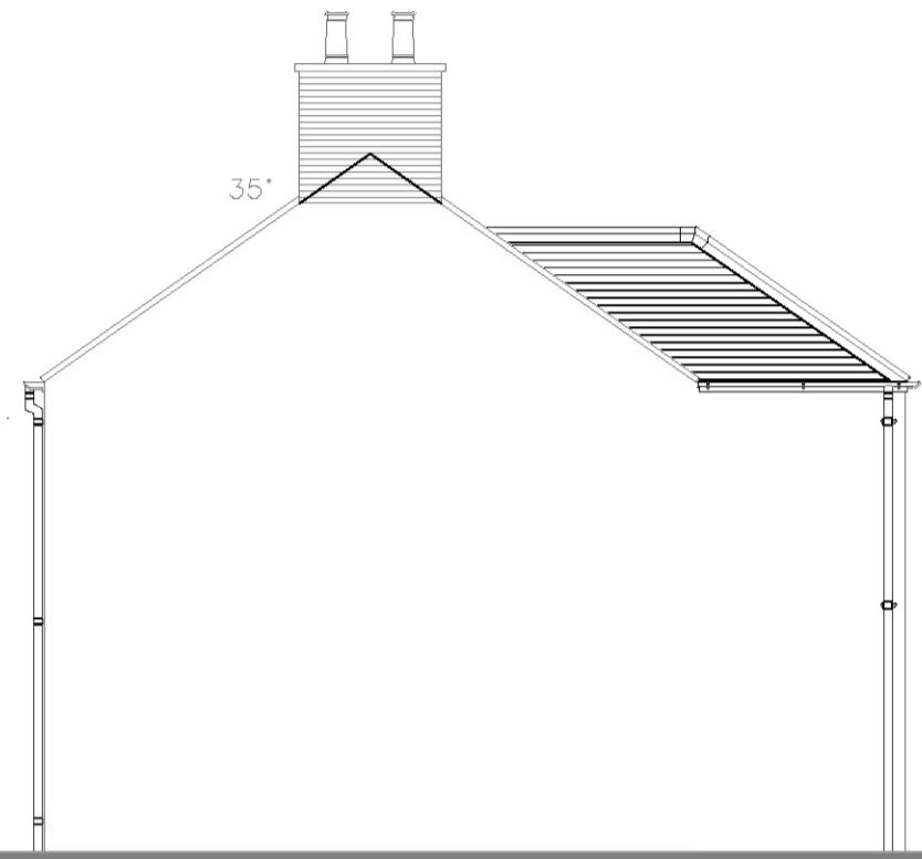
SIDE ELEVATION
