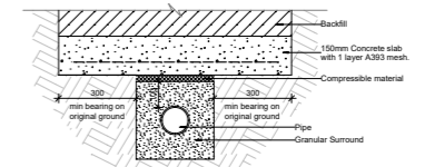
Concrete Protection for Pipes Laid at Shallow Depths Cover < 600mm
