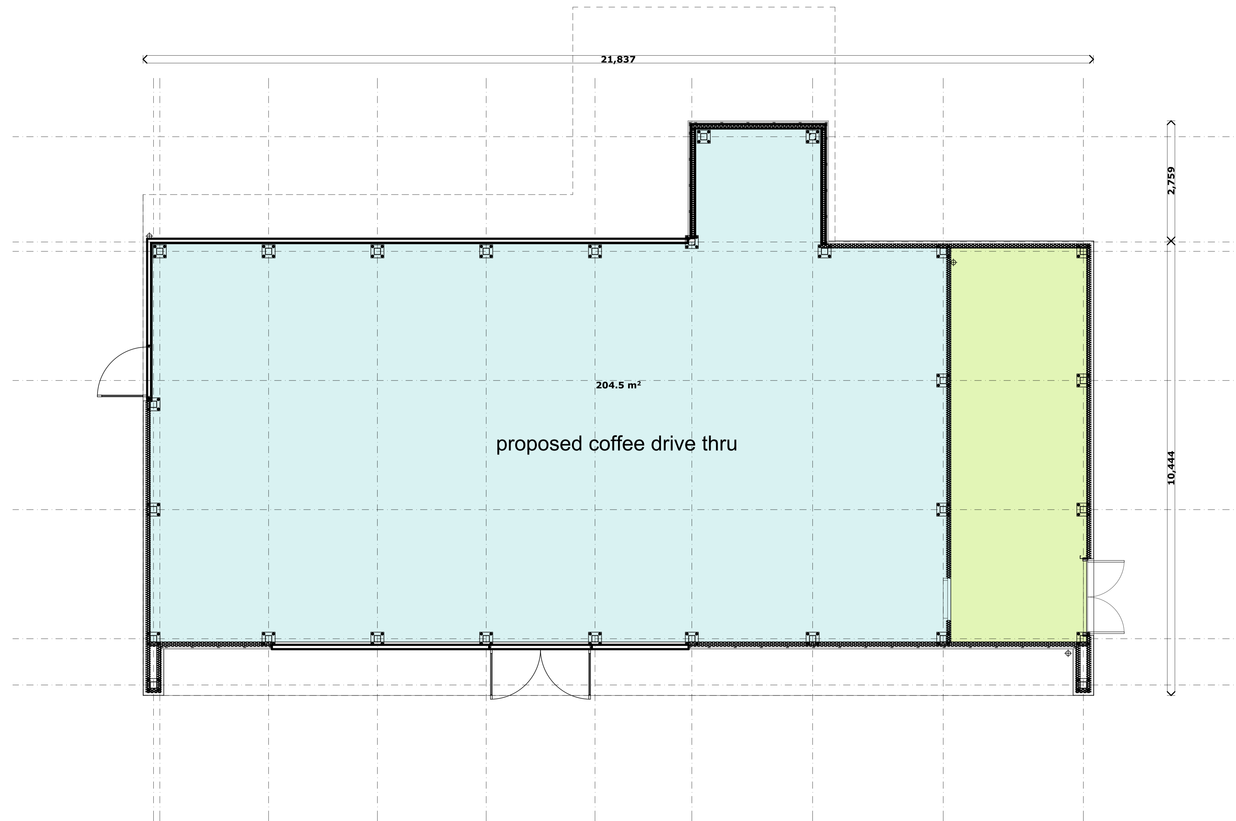
proposed coffee drive thru plan 1:50
