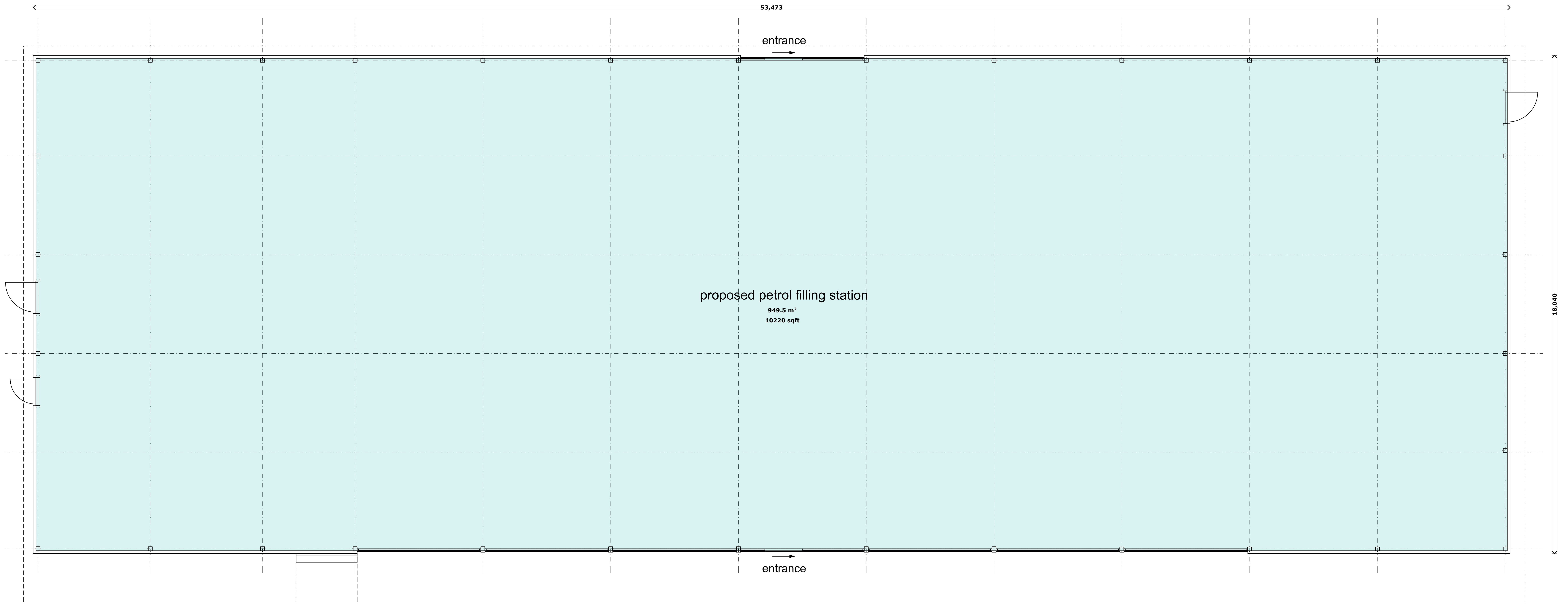
proposed pfs plan 1:50
