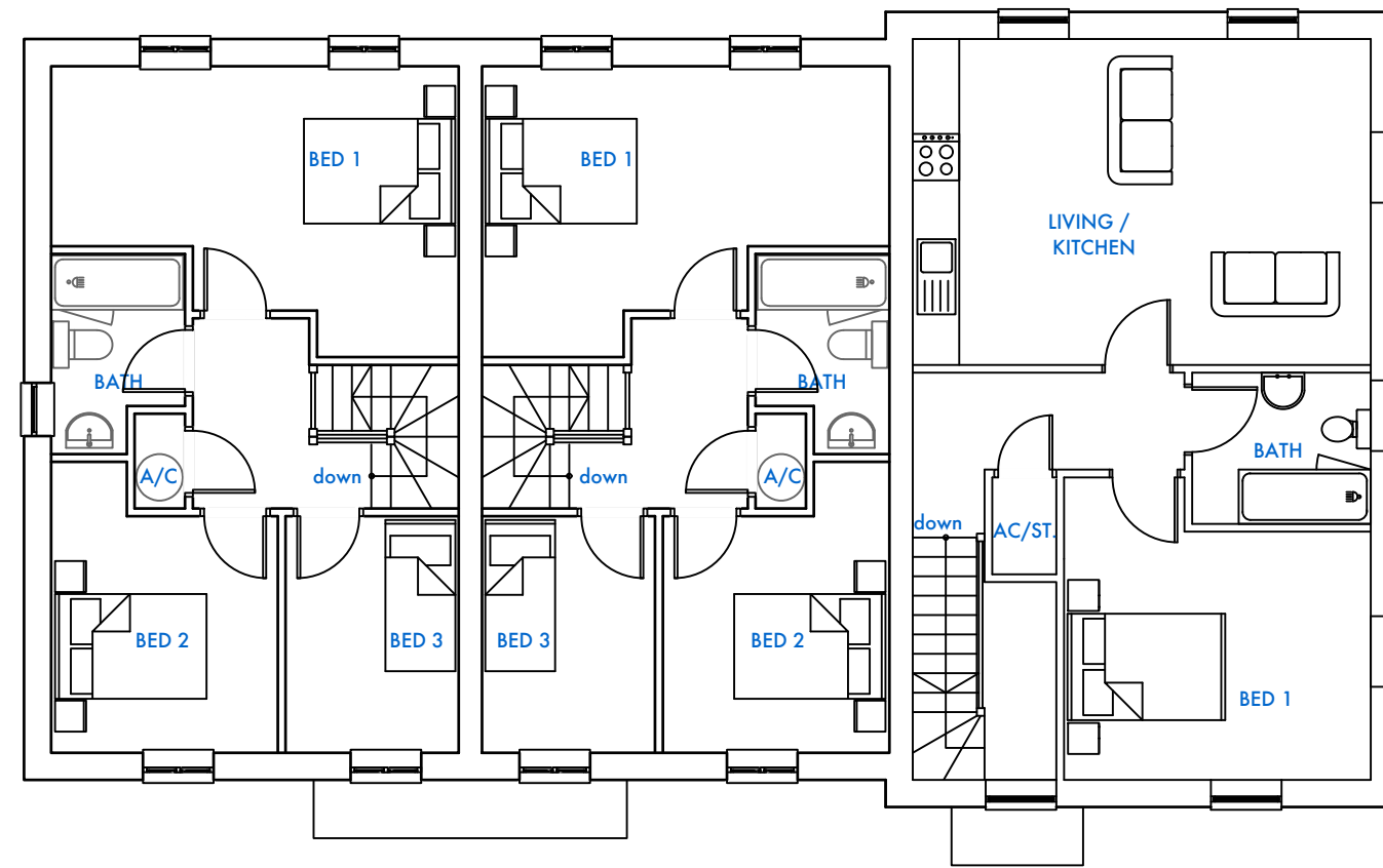
PLOT 18 FIRST FLOOR PLAN
