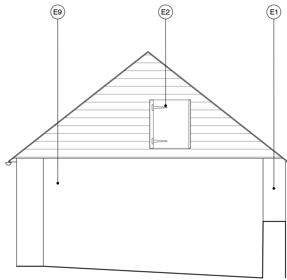
01 Elevation 1 As Existing 1:50
