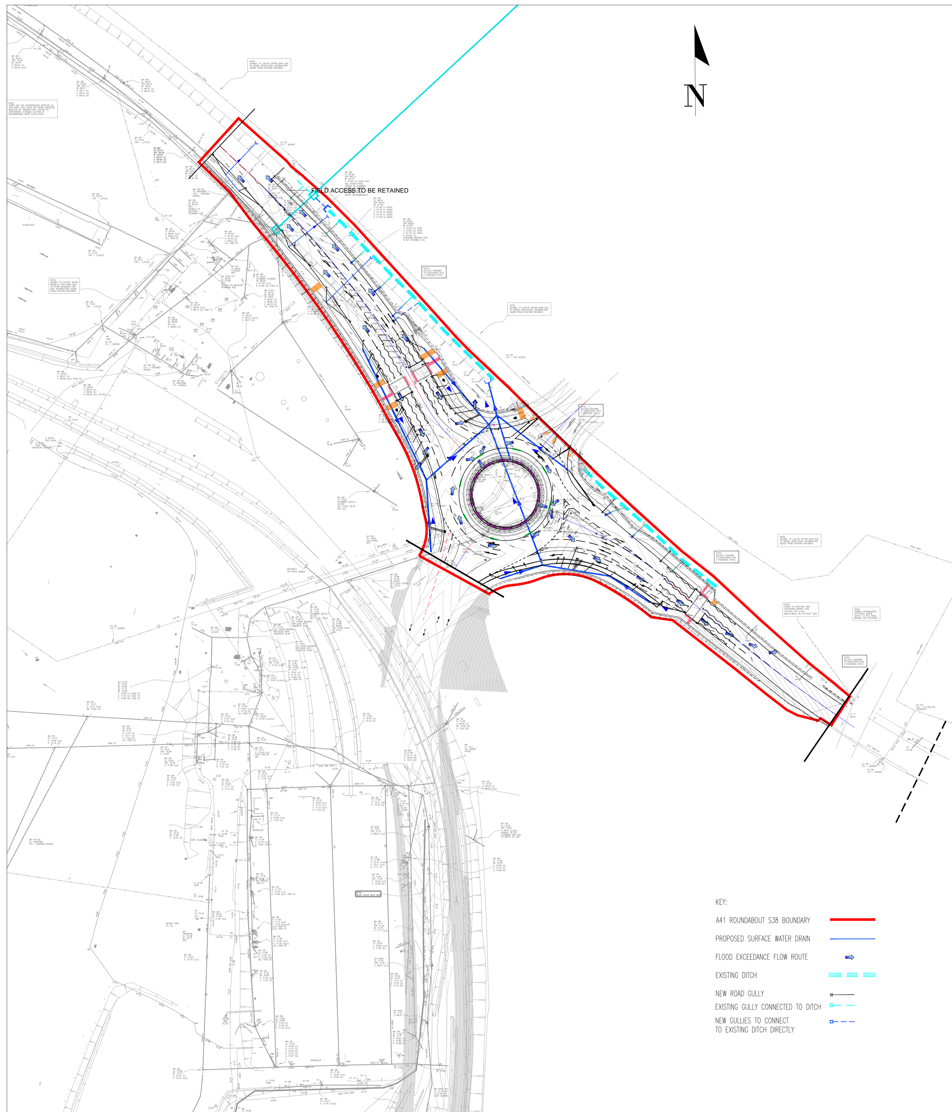
DRAINAGE STRATEGY PLAN
