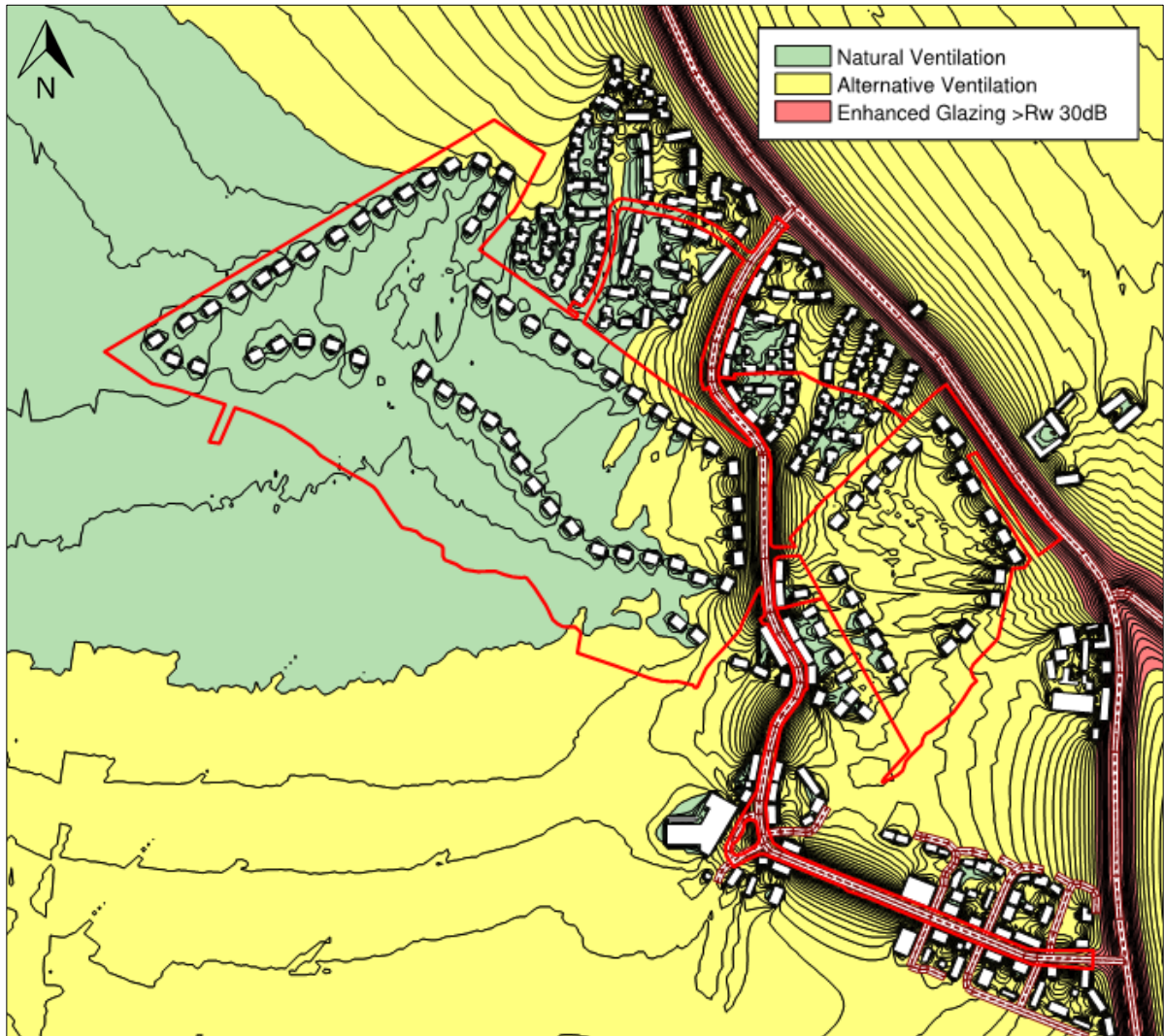
Figure 8.6: Indicative Glazing and Ventilation Strategy – Living Rooms (Grid Height 1.5m)
