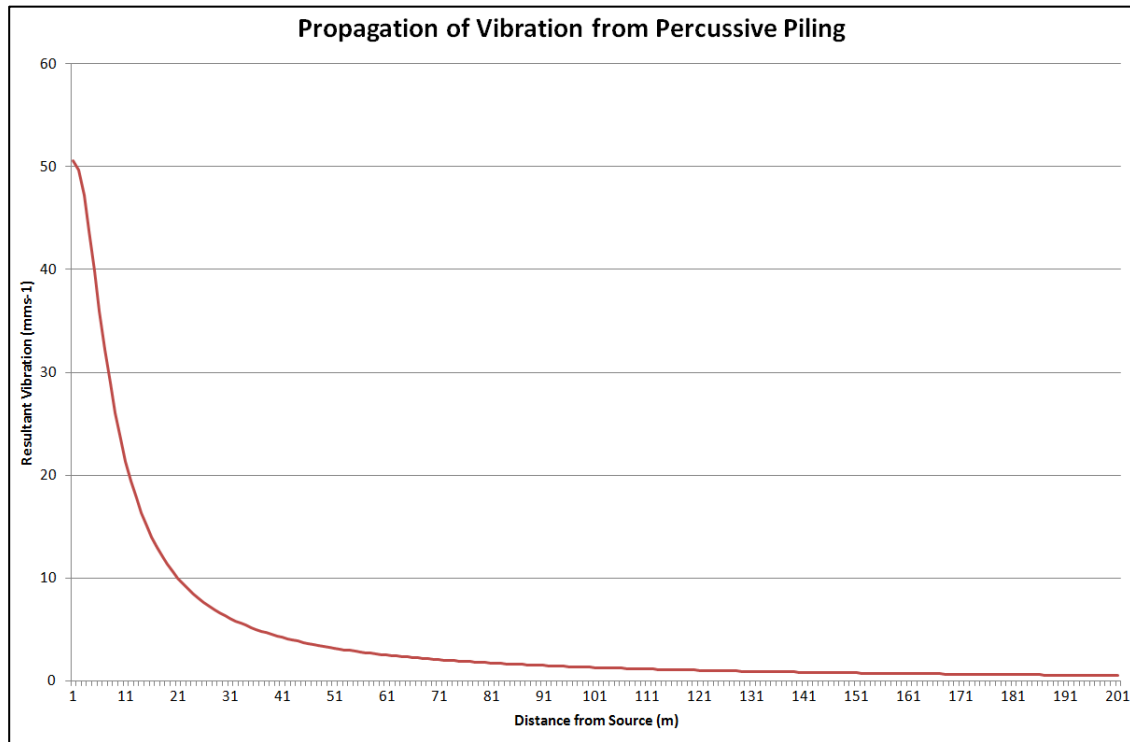
Figure 8.5: Graphical Representation of the Propagation of Vibration from Percussive Piling
