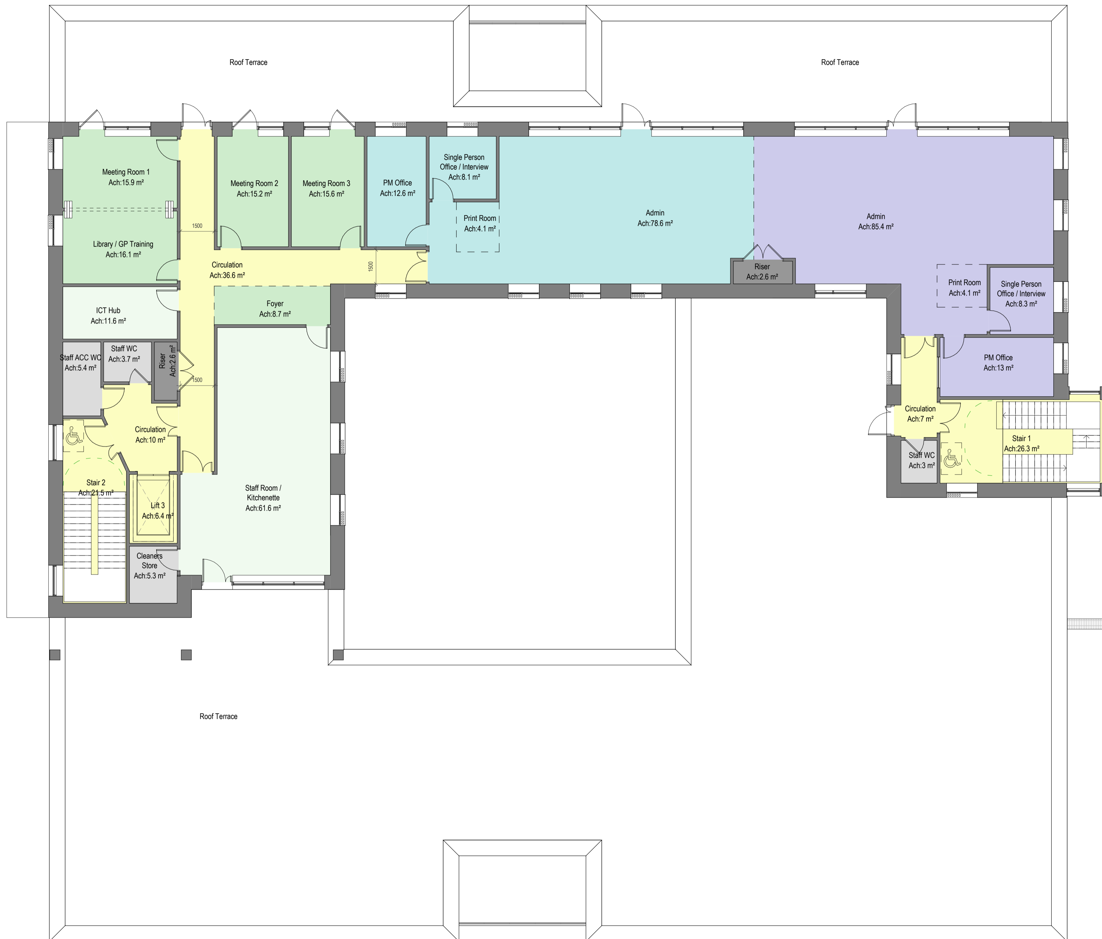
Second Floor Plan 1 : 100
