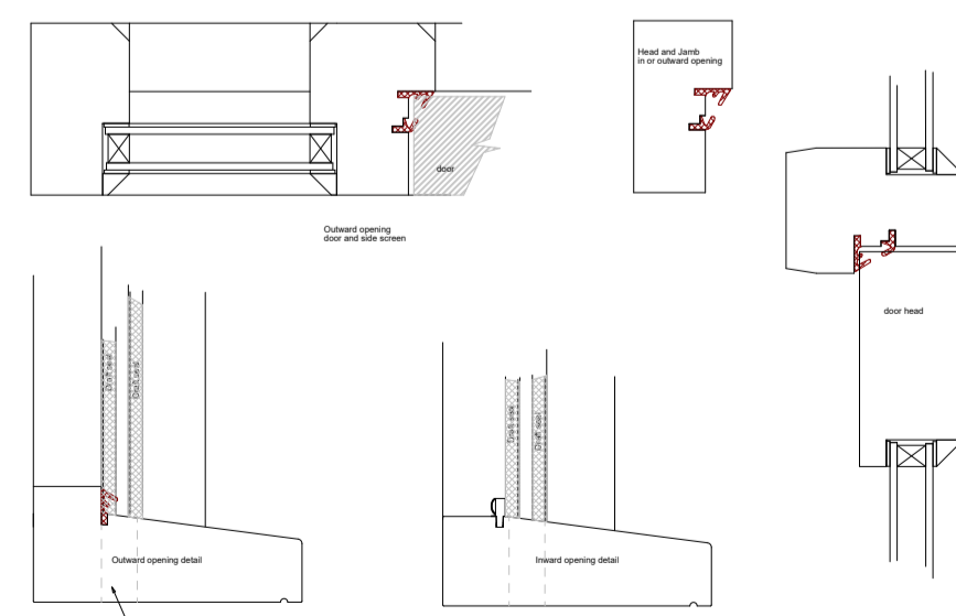
Door and screen details
