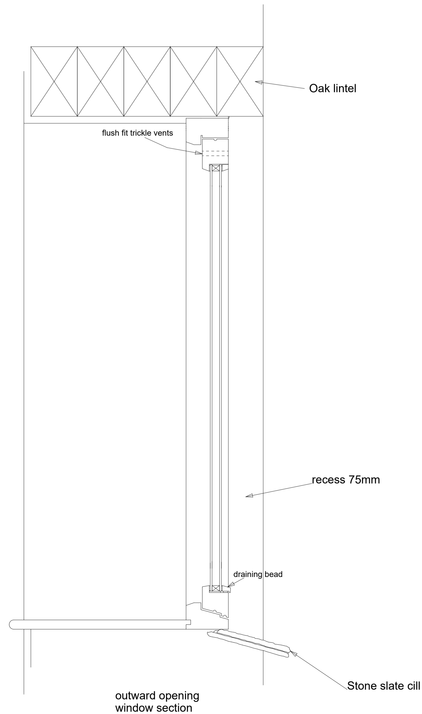
WINDOW SECTION
