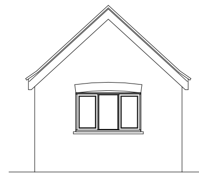
SOUTH WEST ELEVATION
