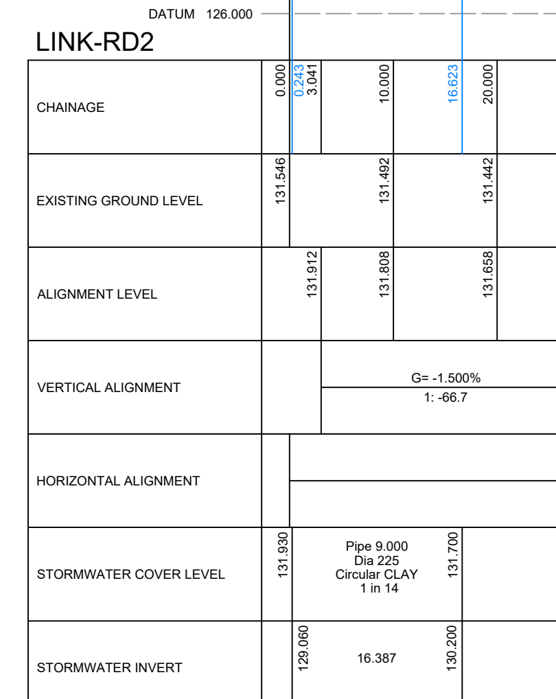
DRAINAGE SECTION - MH S14 TO S13
