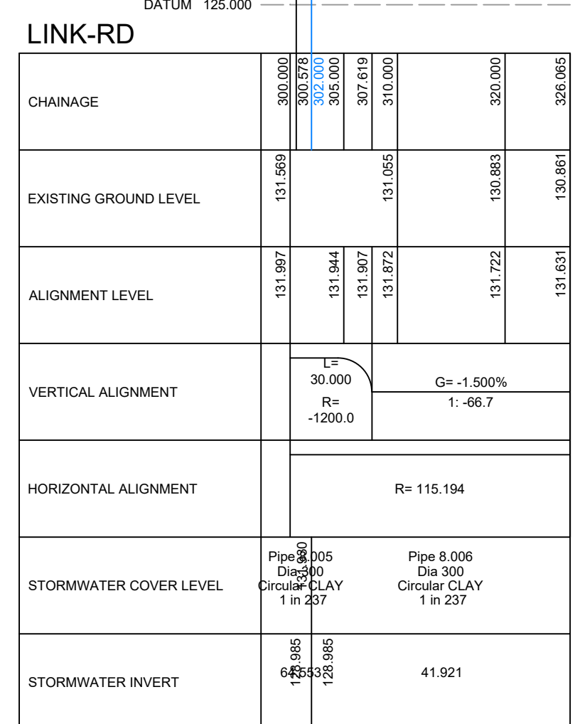
DRAINAGE SECTION - MH S14
