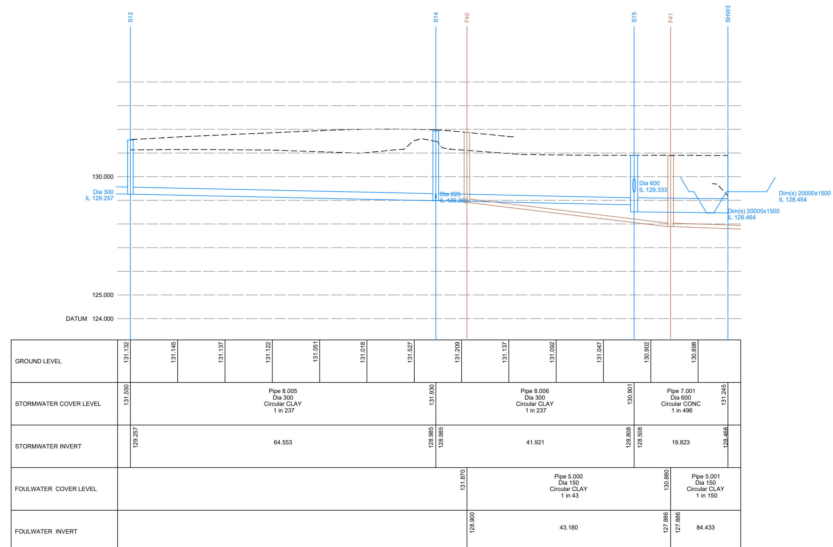
DRAINAGE SECTION - MH S12 TO SHW3, F40 TO F41
