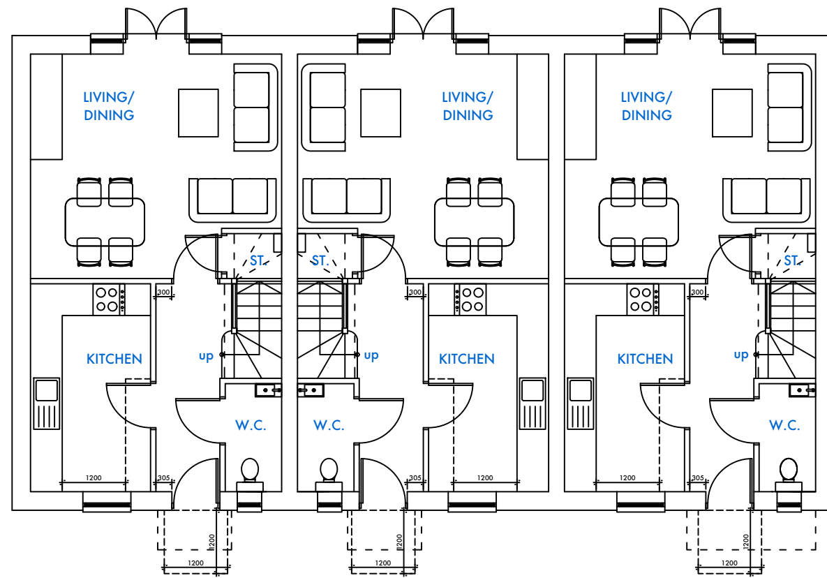
PLOT 21 PLOT 20 PLOT 19 GROUND FLOOR PLAN
