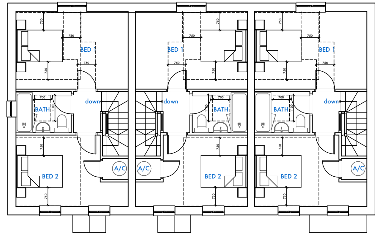
PLOT 21 PLOT 20 PLOT 19 FIRST FLOOR PLAN
