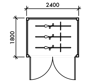
GARDEN SHED PLAN
