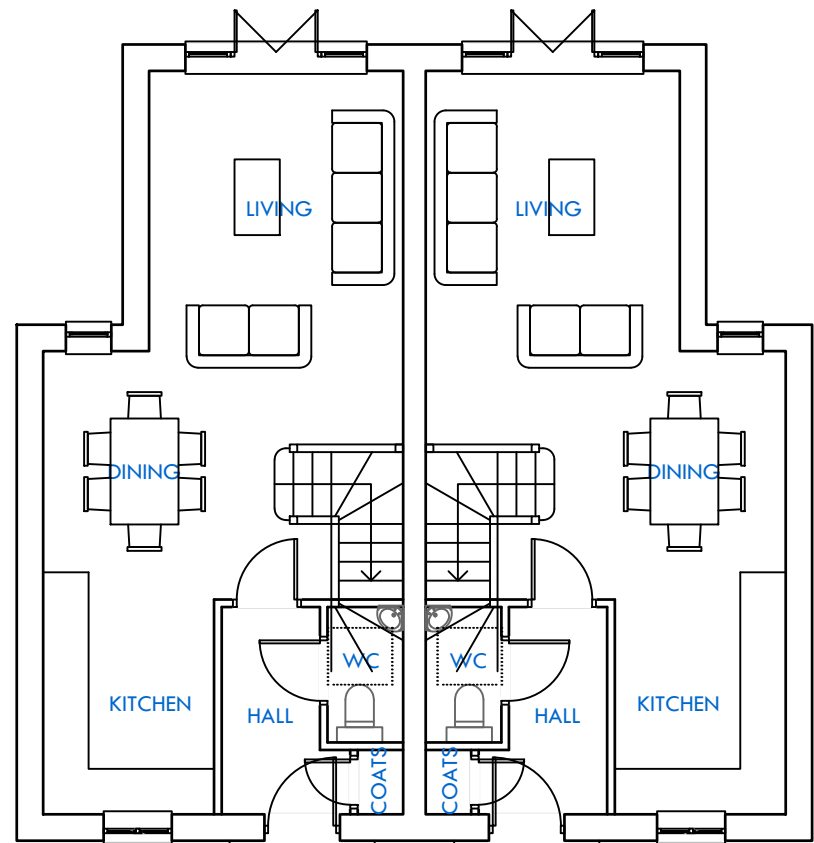
PLOT 11 PLOT 12 GROUND FLOOR PLAN
