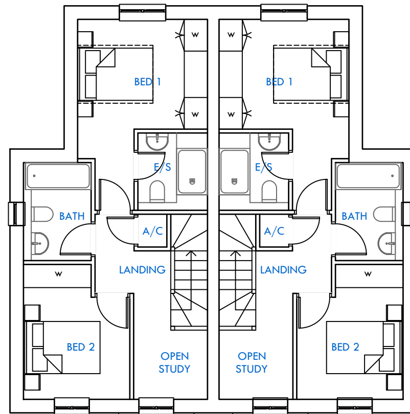
PLOT 11 PLOT 12 FIRST FLOOR PLAN
