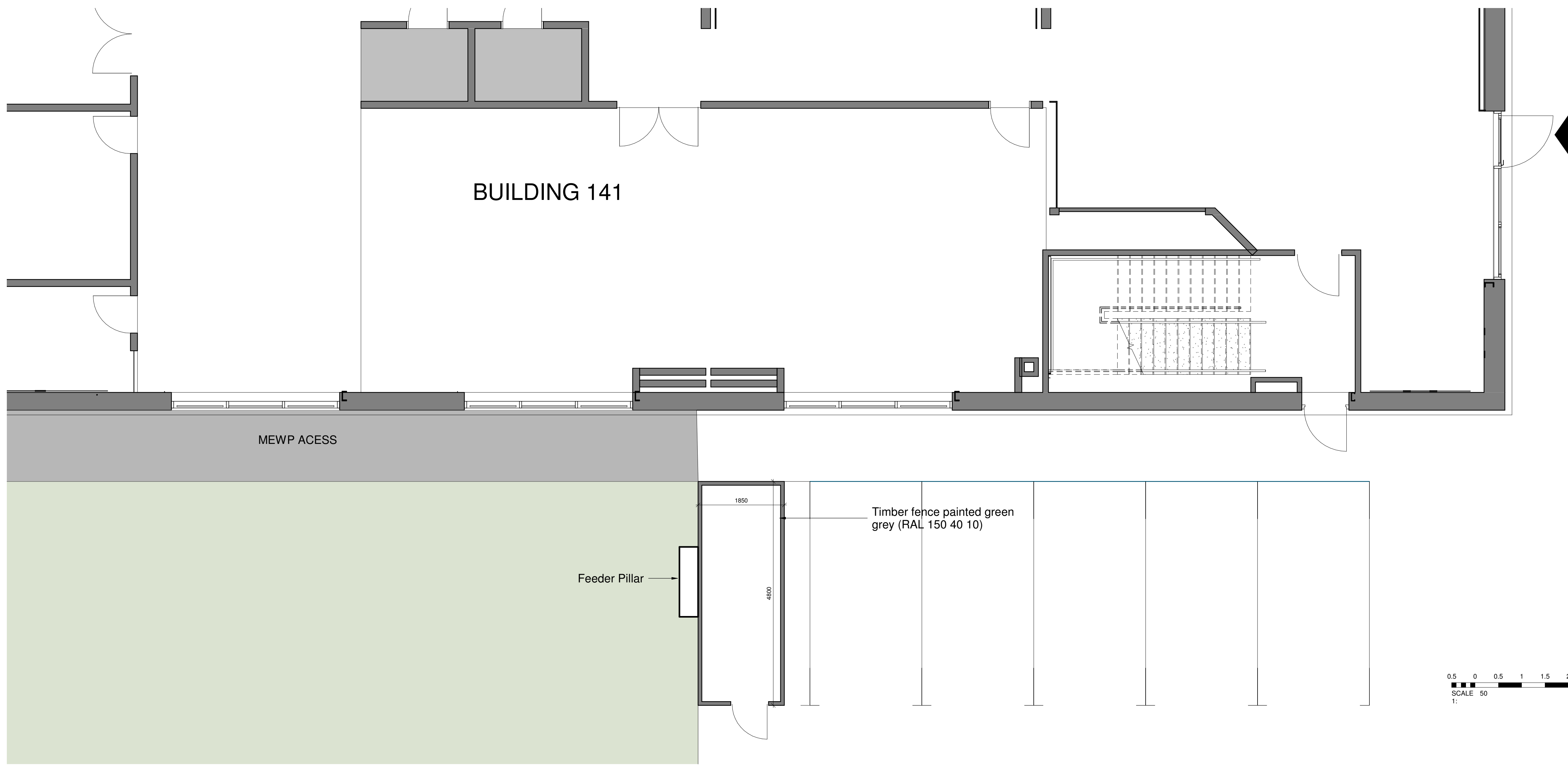
00_Ground Floor - External Plant Store 1 : 50
