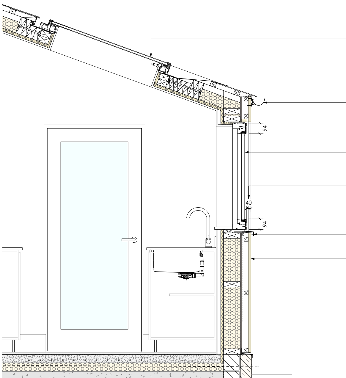
DETAIL 04 UTILITY WINDOW DETAILS SECTION 1:20
