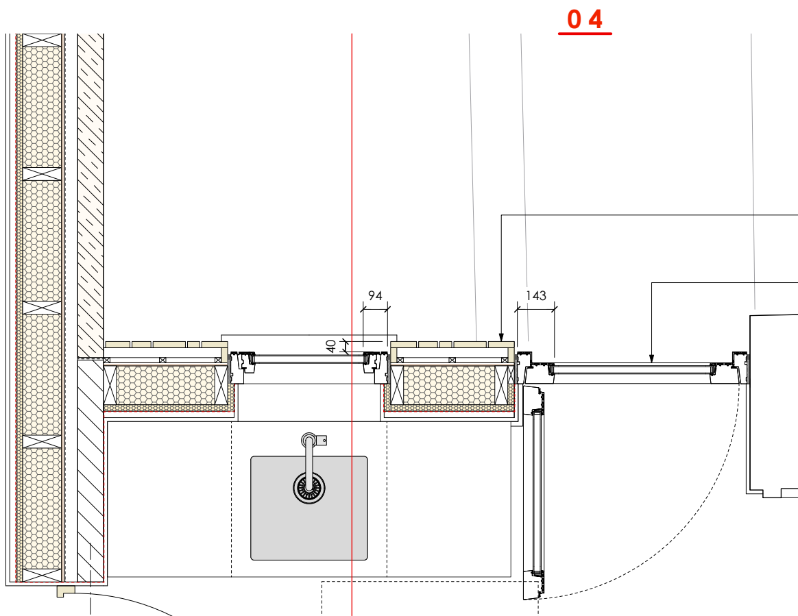
DETAIL 03 UTILITY WINDOW + DOOR DETAILS GROUND FLOOR PLAN 1:20
