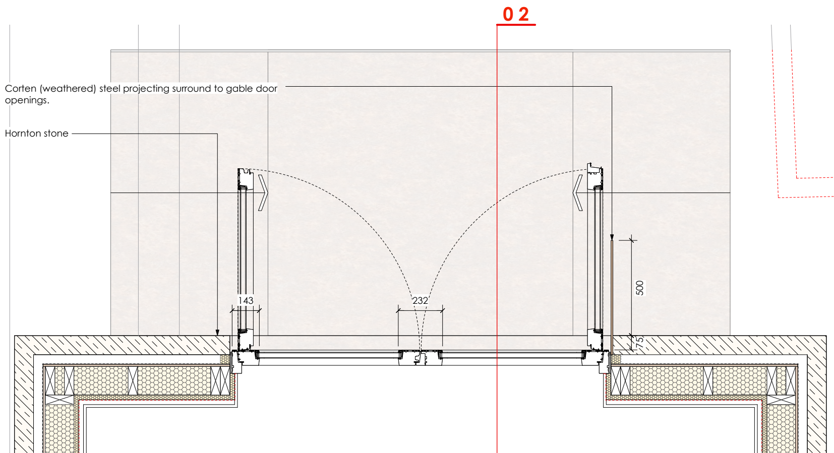
DETAIL 01 TYPICAL DOOR DETAILS GROUND FLOOR PLAN 1:20
