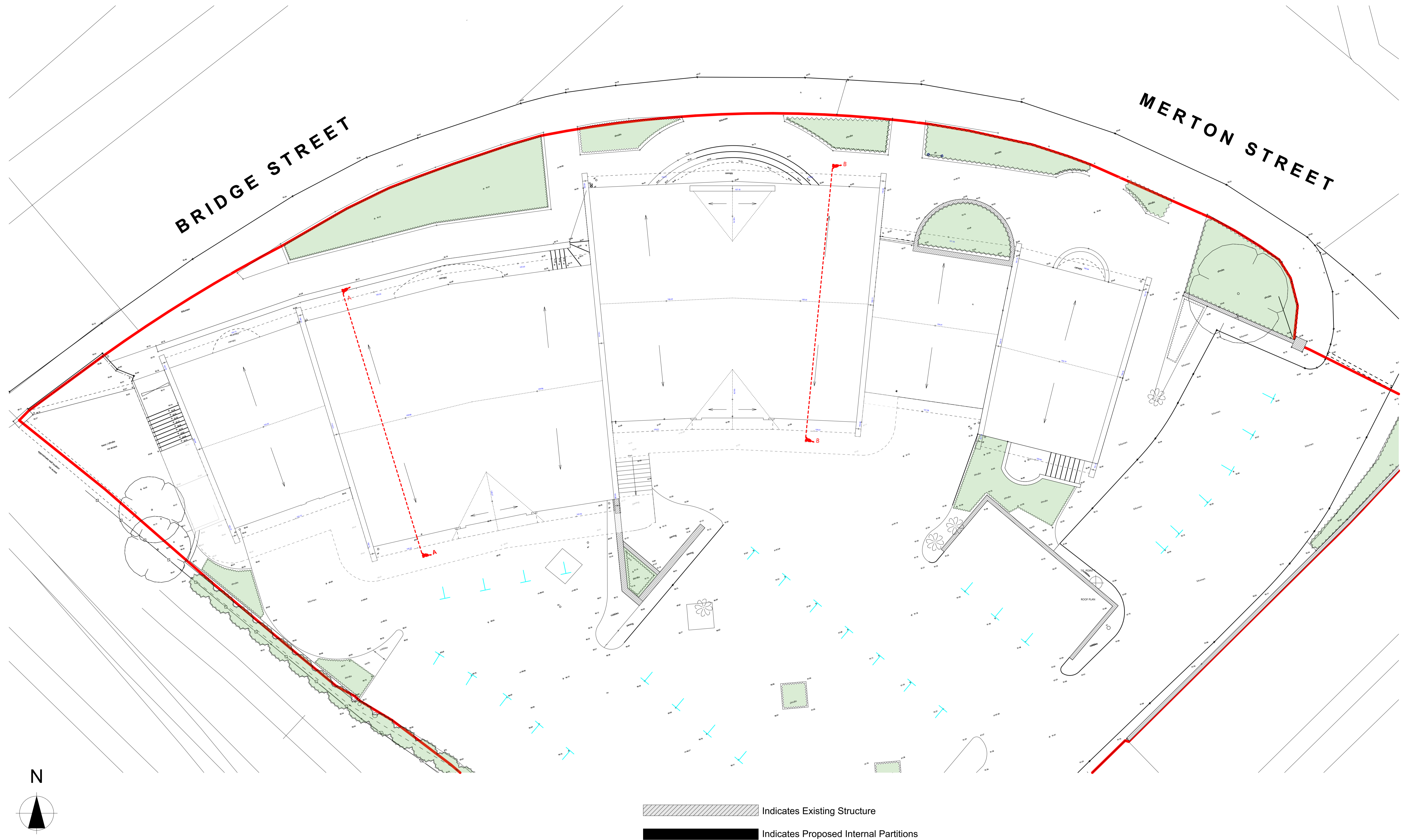
PROPOSED ROOF PLAN - SCALE 1:100 @ A1
