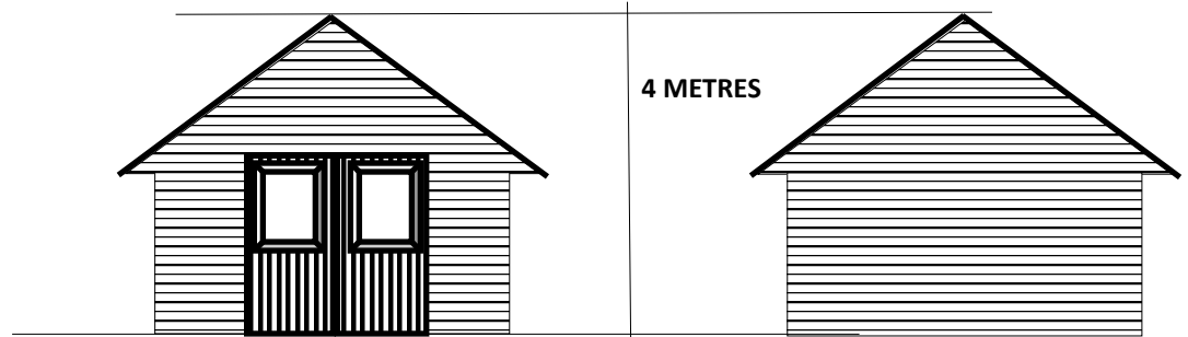
WESTERN ELEVATION
